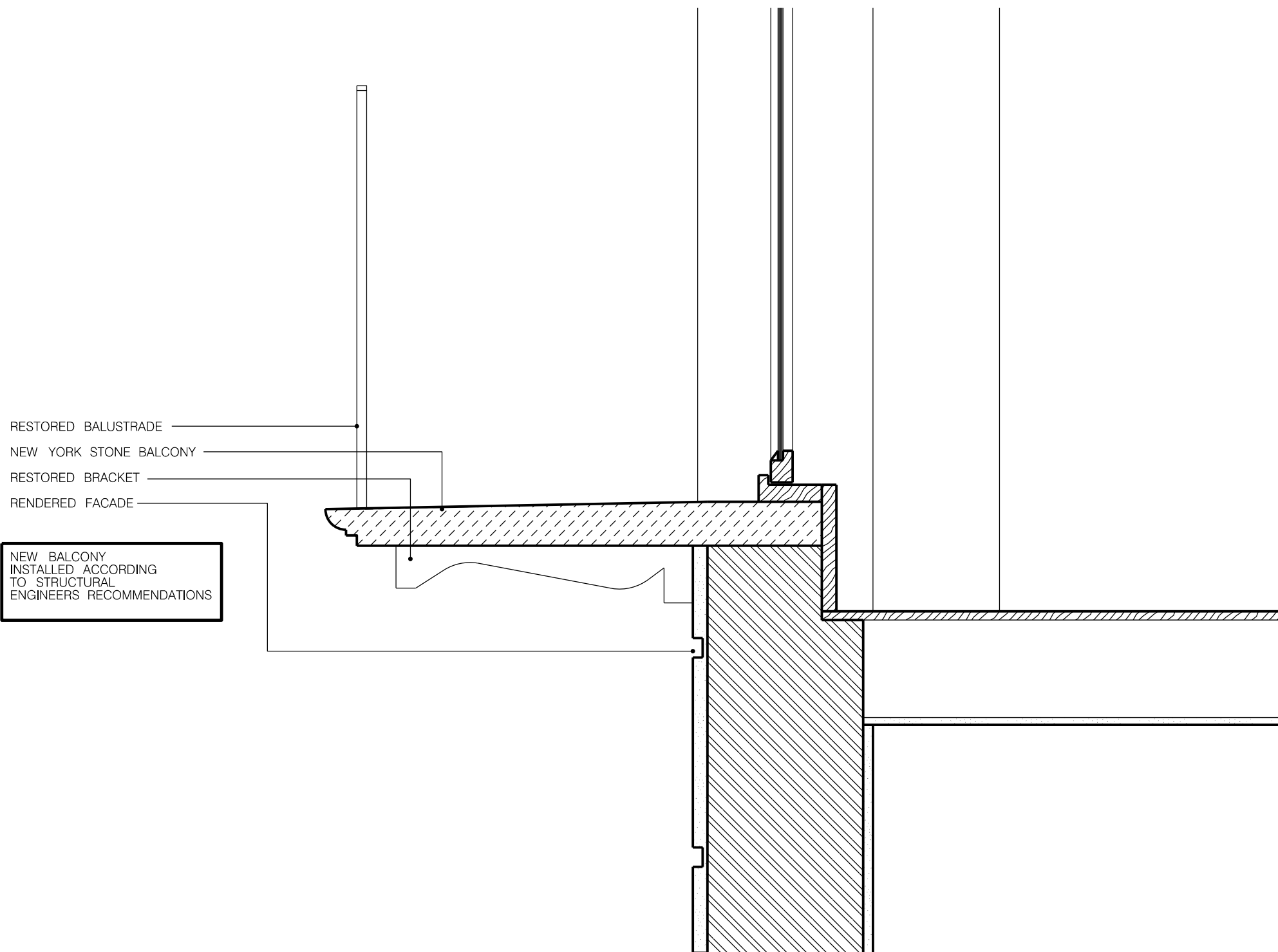
SECTION DETAIL THROUGH BALCONY
