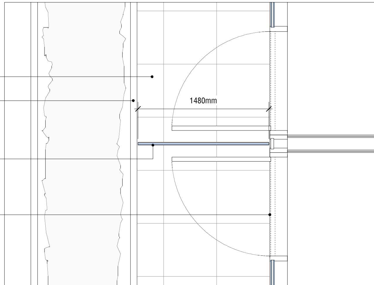
DETAIL PLAN OF GLASS SCREEN
