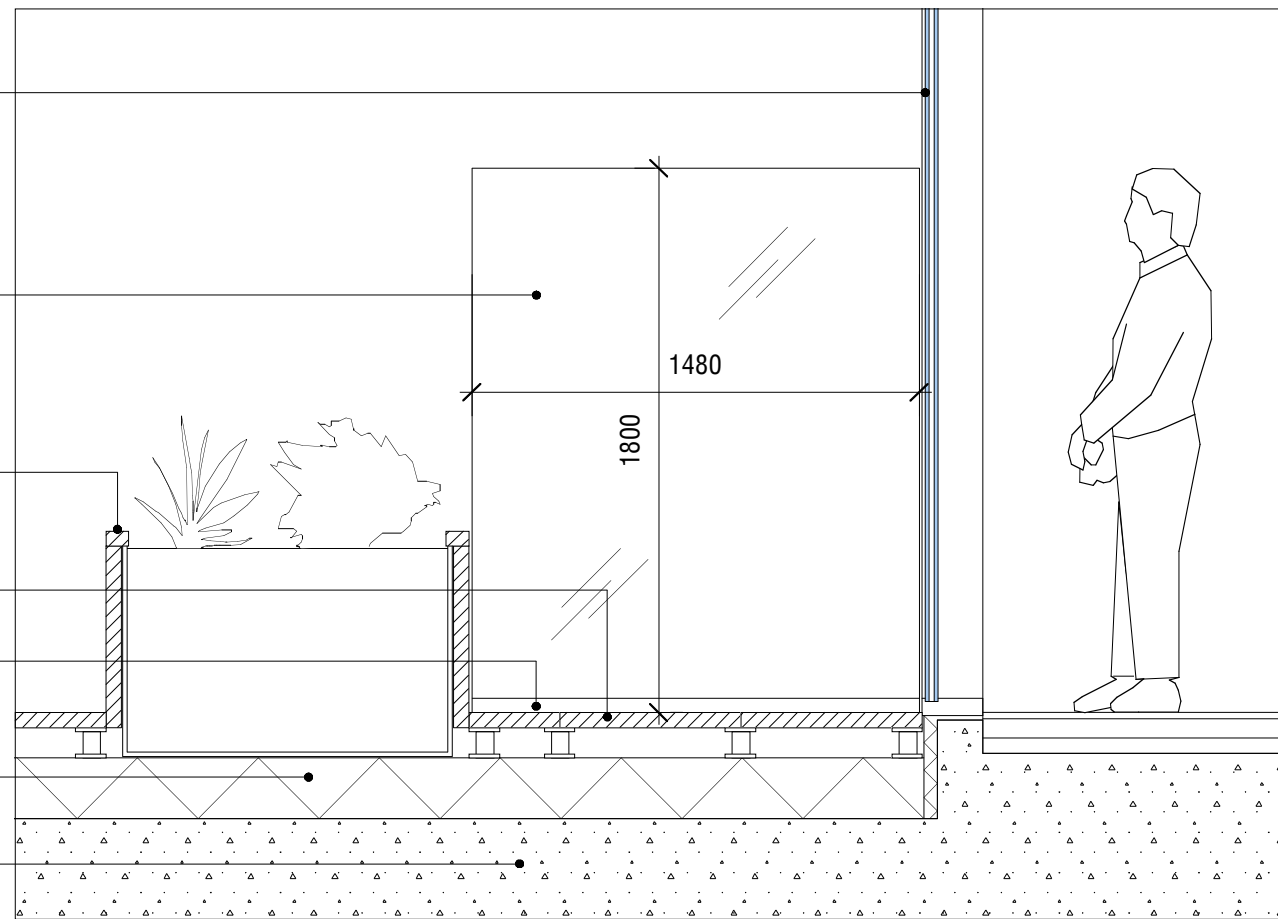
DETAIL SECTION THROUGH TERRACE SHOWING ELEVATION OF GLASS SCREEN
