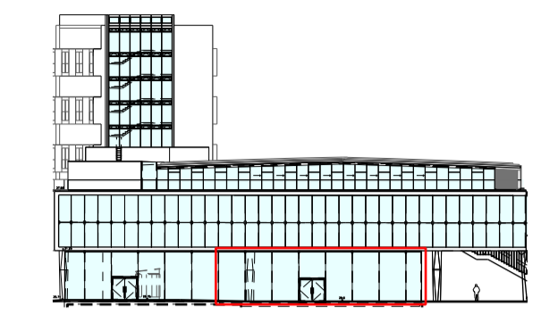
Location Elevation- North
