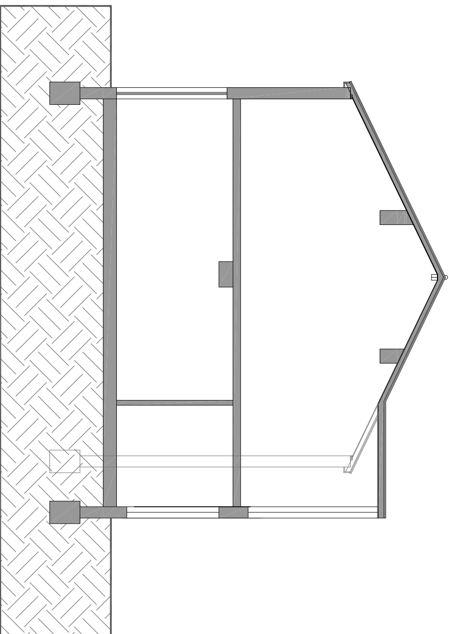
SECTION C-C
