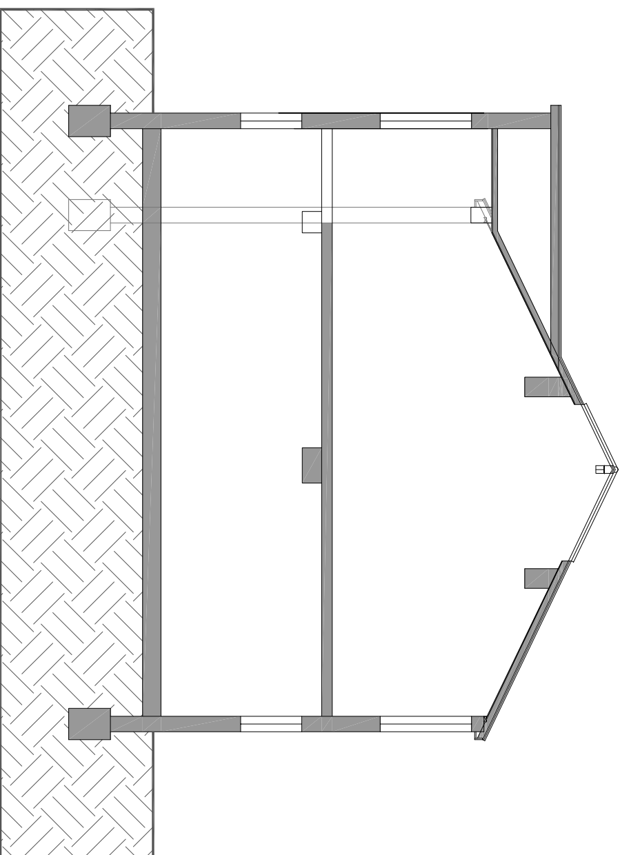
SECTION B-B
