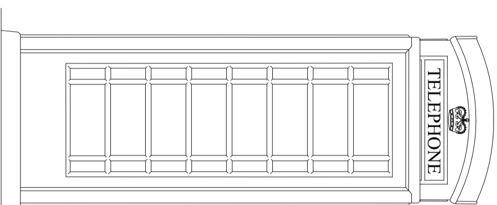
Existing Side Elevation 1 @ 1 : 20
