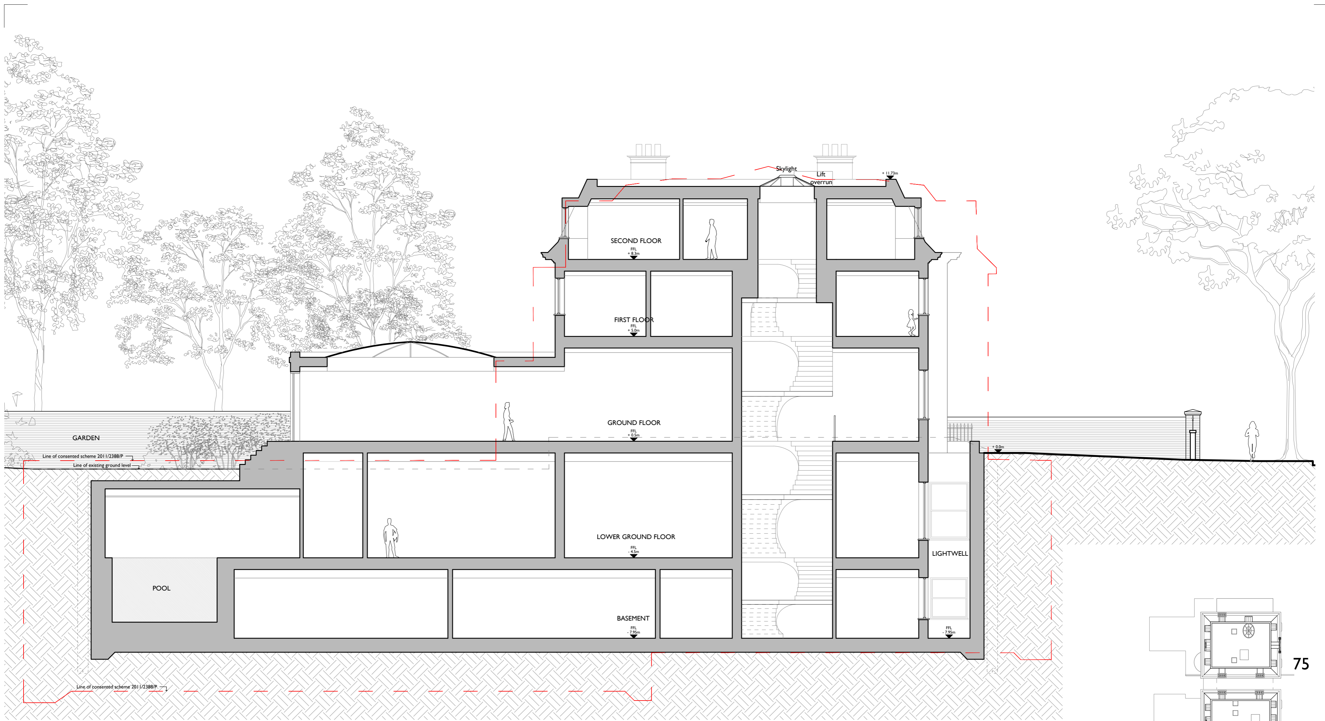
1 Proposed Section DD: 73 Avenue Road 219 1:100 @ A2
