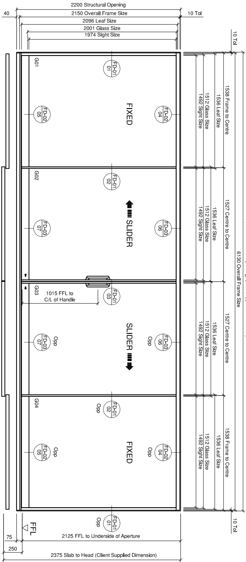
6150 Structural Opening (Site Supplied Dimension) 6130 Overall Frame Size
