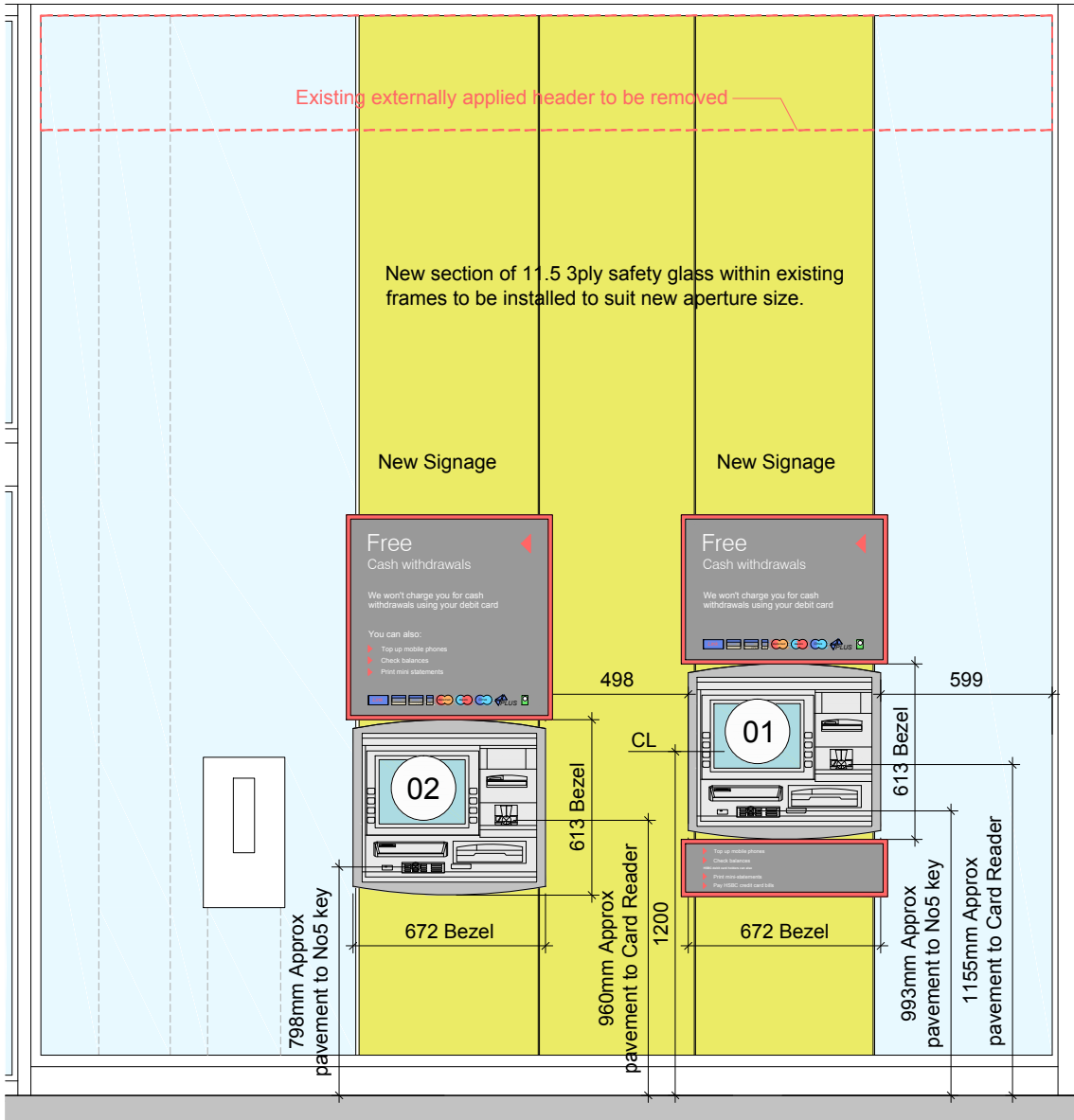
Proposed Detailed Elevation of Affected Area (scale 1:25 @ A3)
