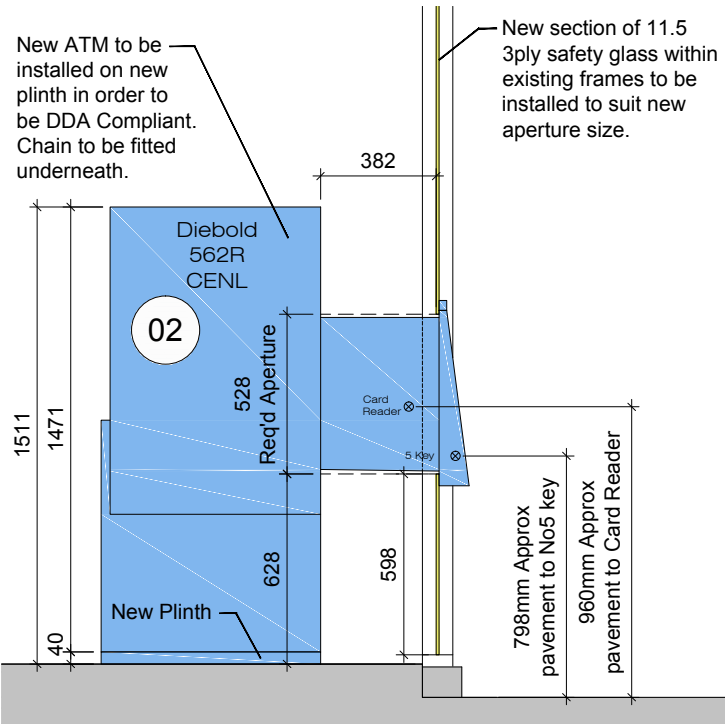
Proposed Section - ATM No2 (scale 1:25 @ A3)
