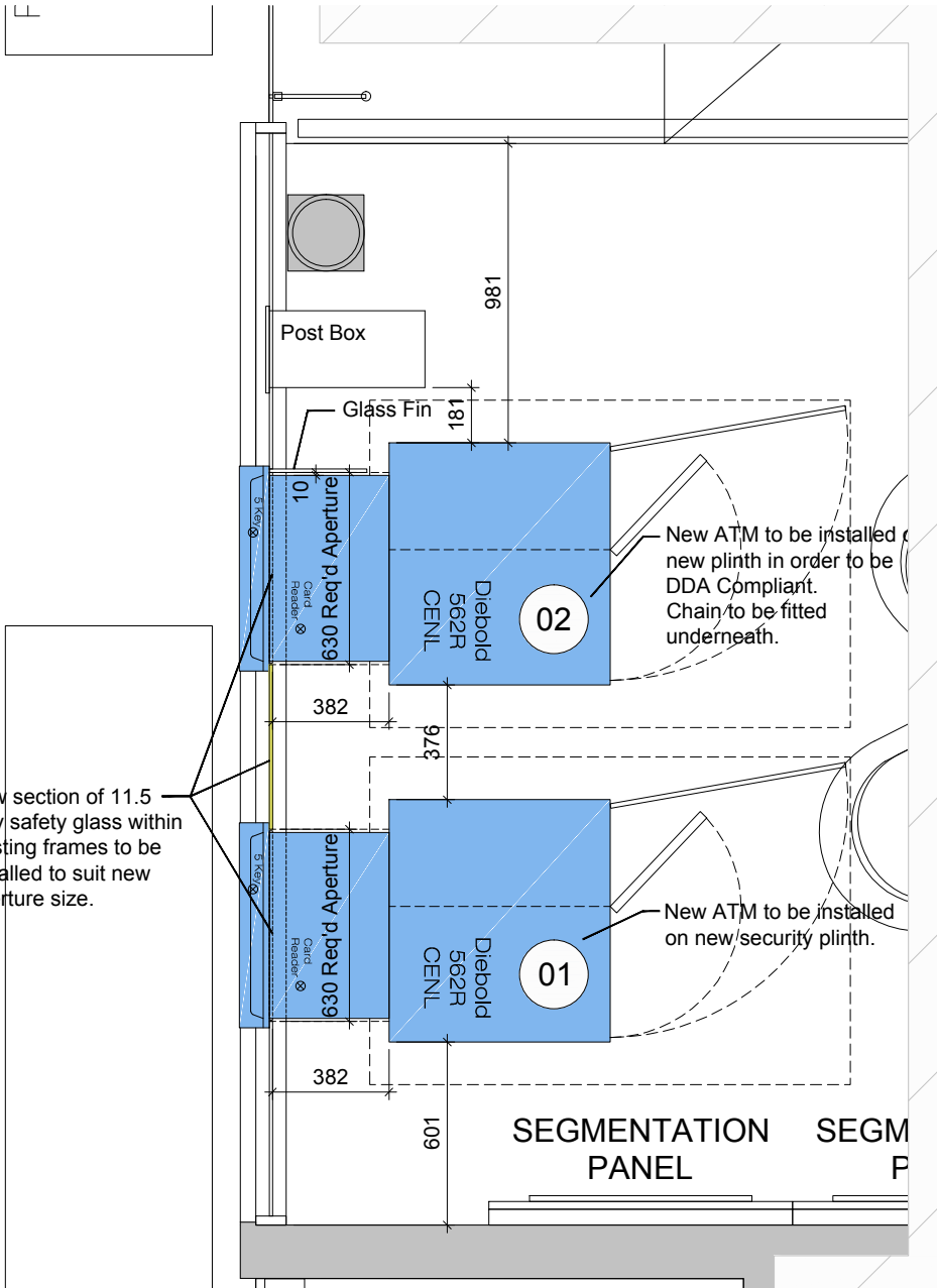
Proposed Detailed Plan of Affected Area (scale 1:25 @ A3)
