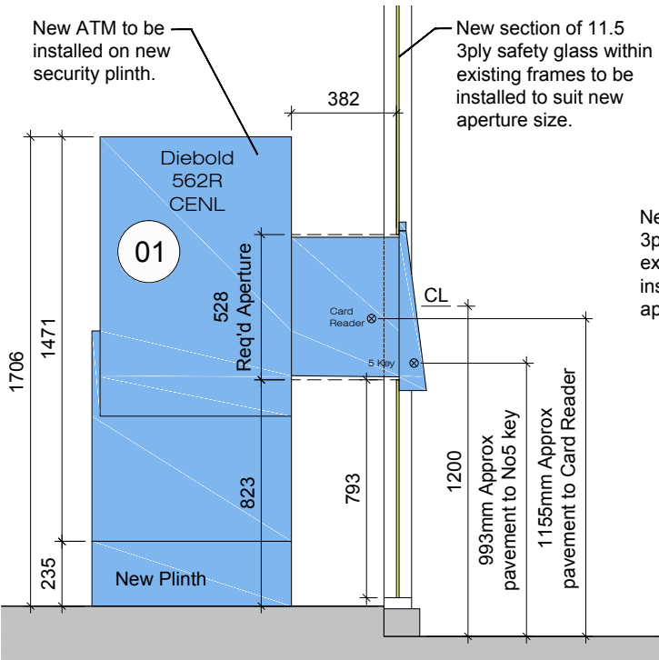
Proposed Section - ATM No1 (scale 1:25 @ A3)
