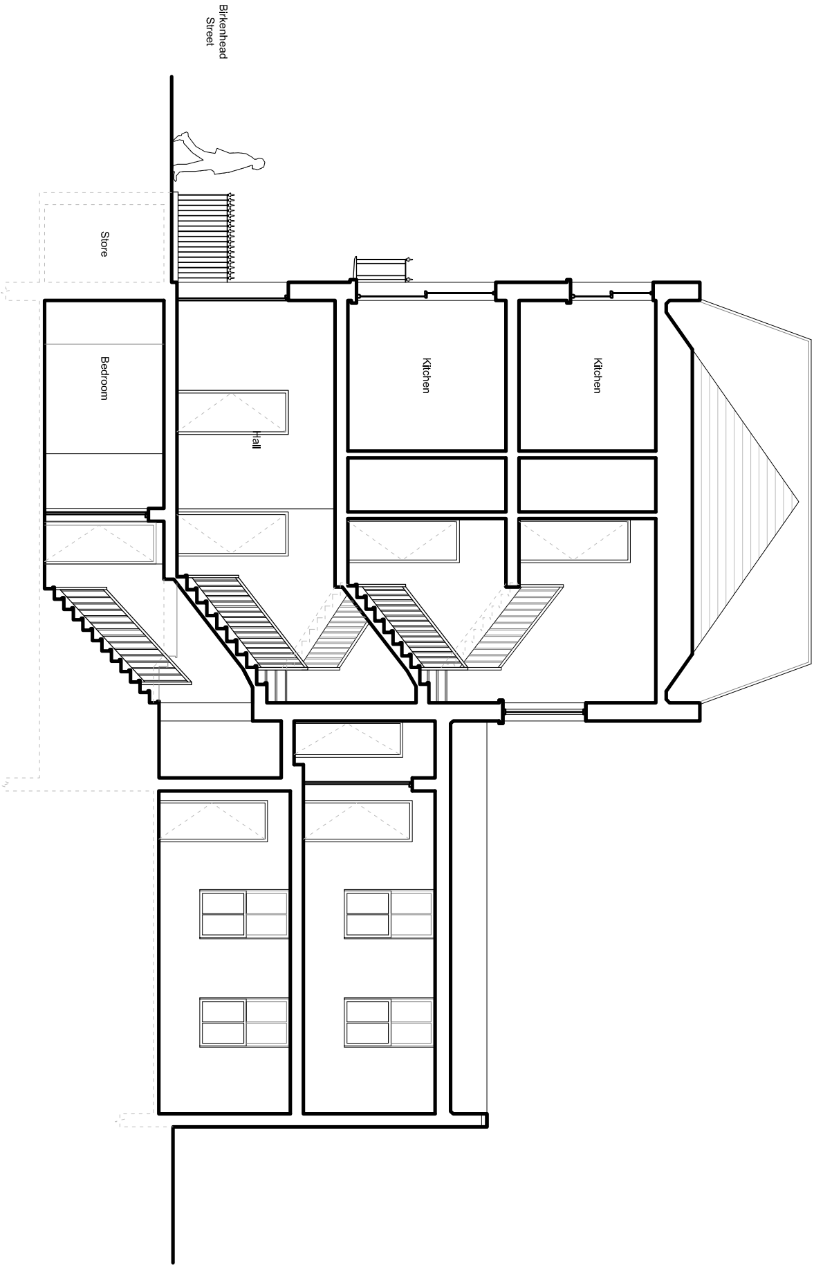
EXISTING SECTION AA
