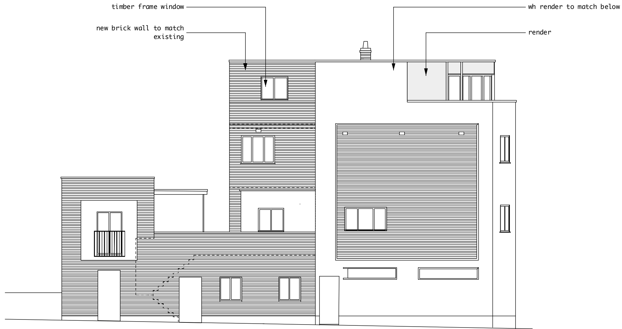
1 proposed Gilden Crescent elevation Scale: 1:100
