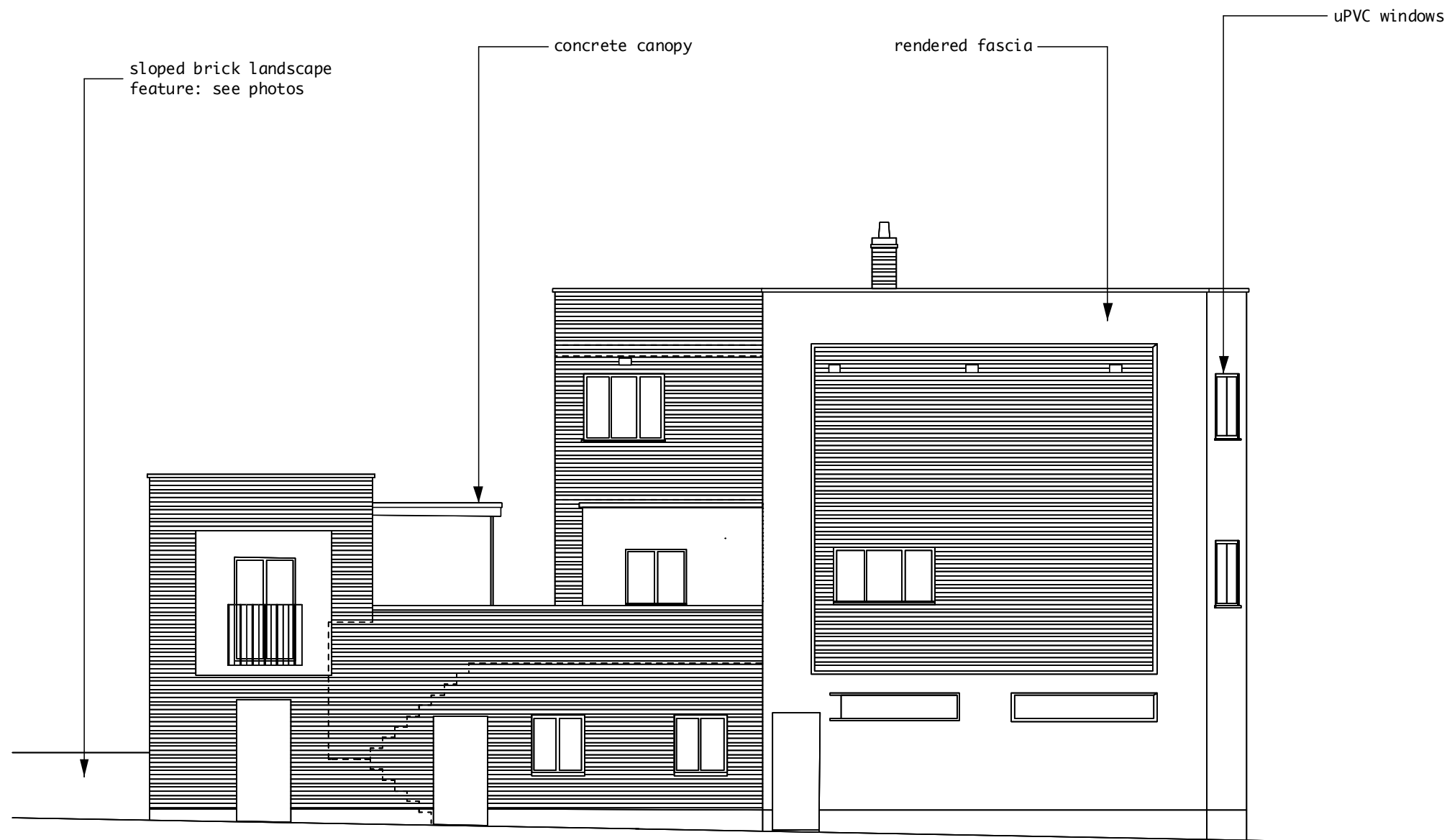
1 existing Gilden Crescent elevation Scale: 1:100
