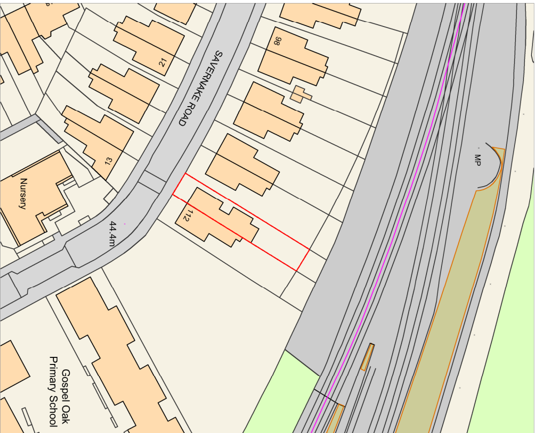
EXISTING SITE LOCATION PLAN SCALE 1:1250
