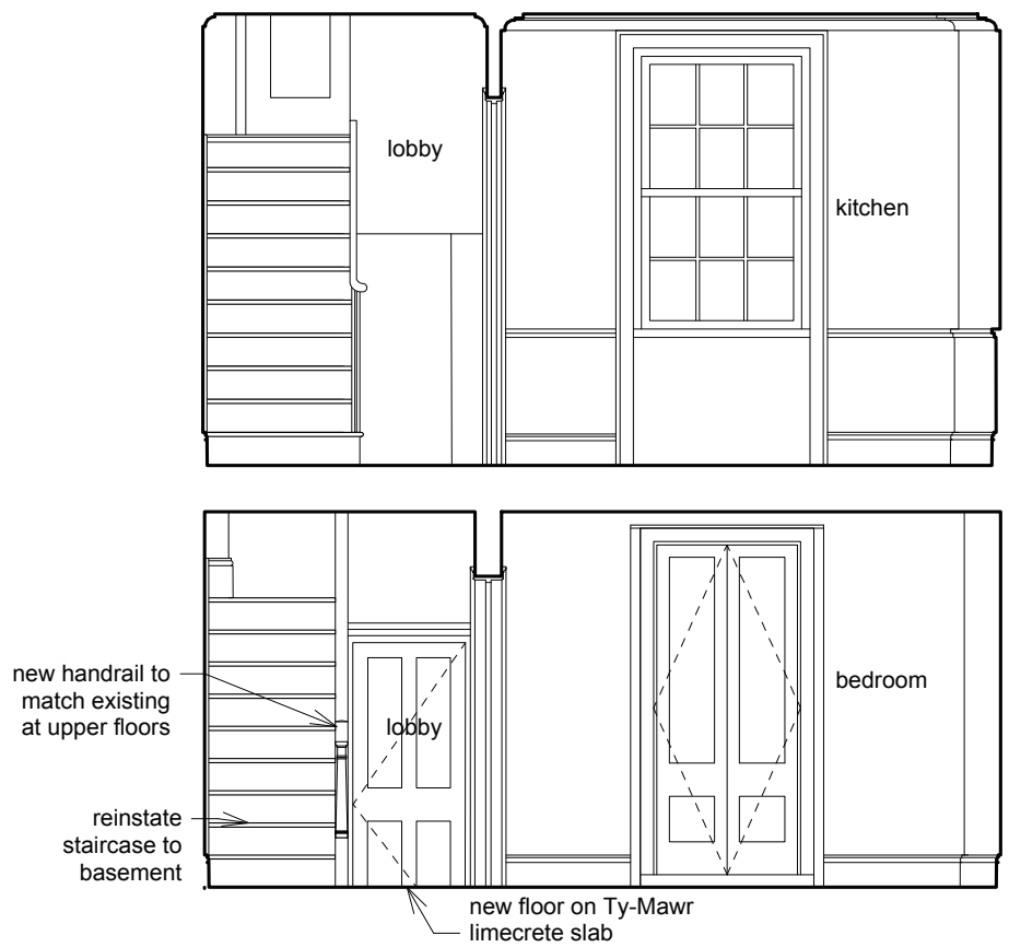
B Section B 12 1:50@A3
