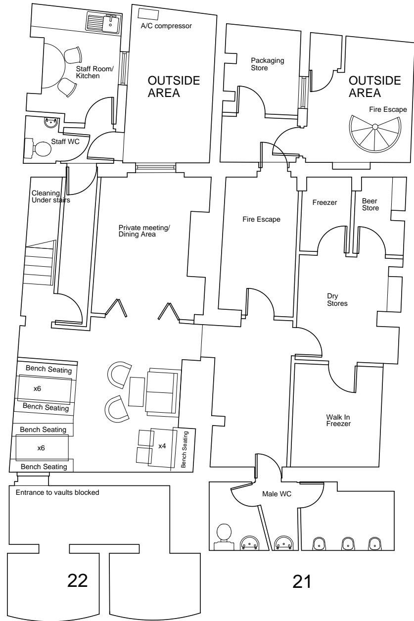
BASEMENT PLAN 1:100
