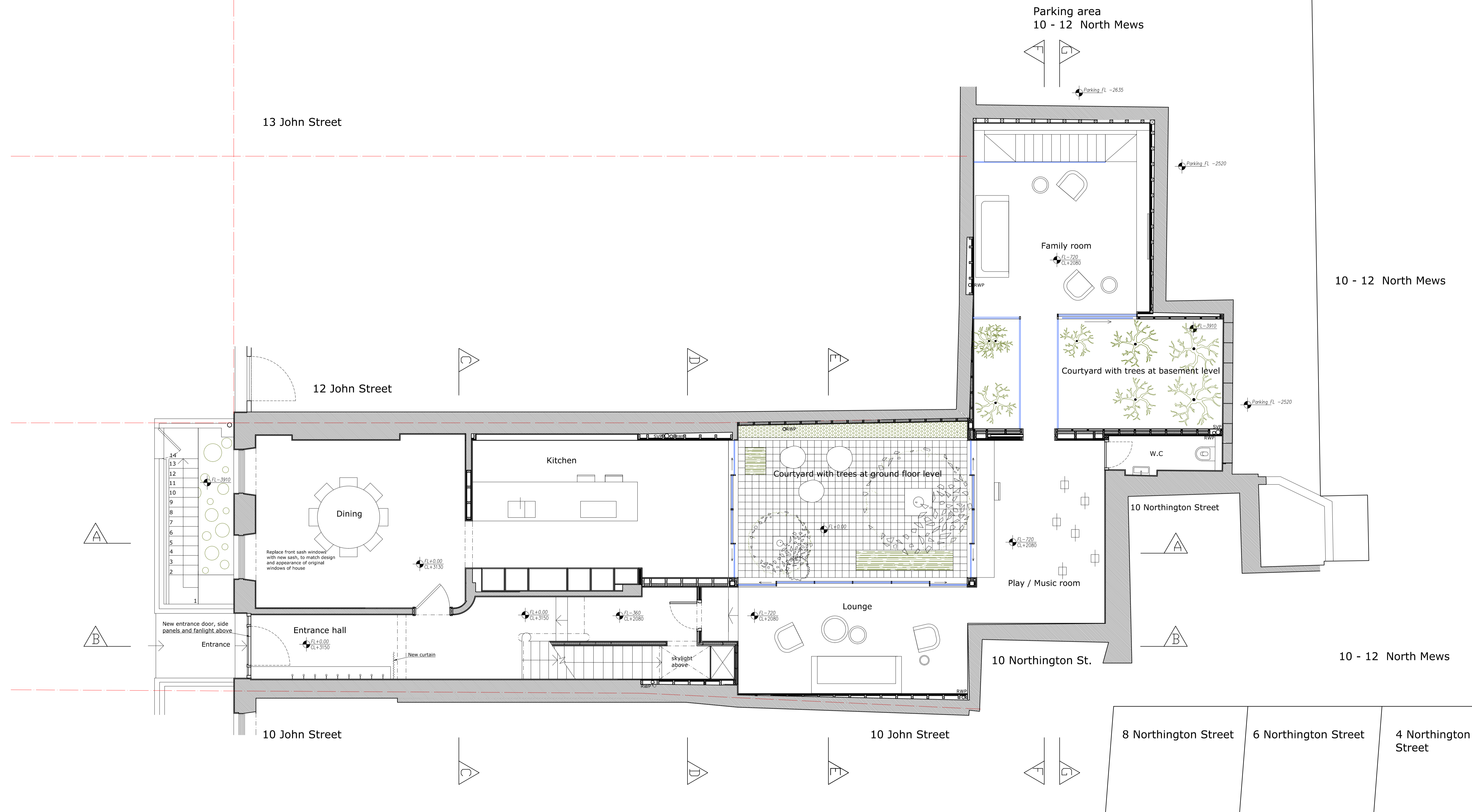
Proposed Ground Floor
