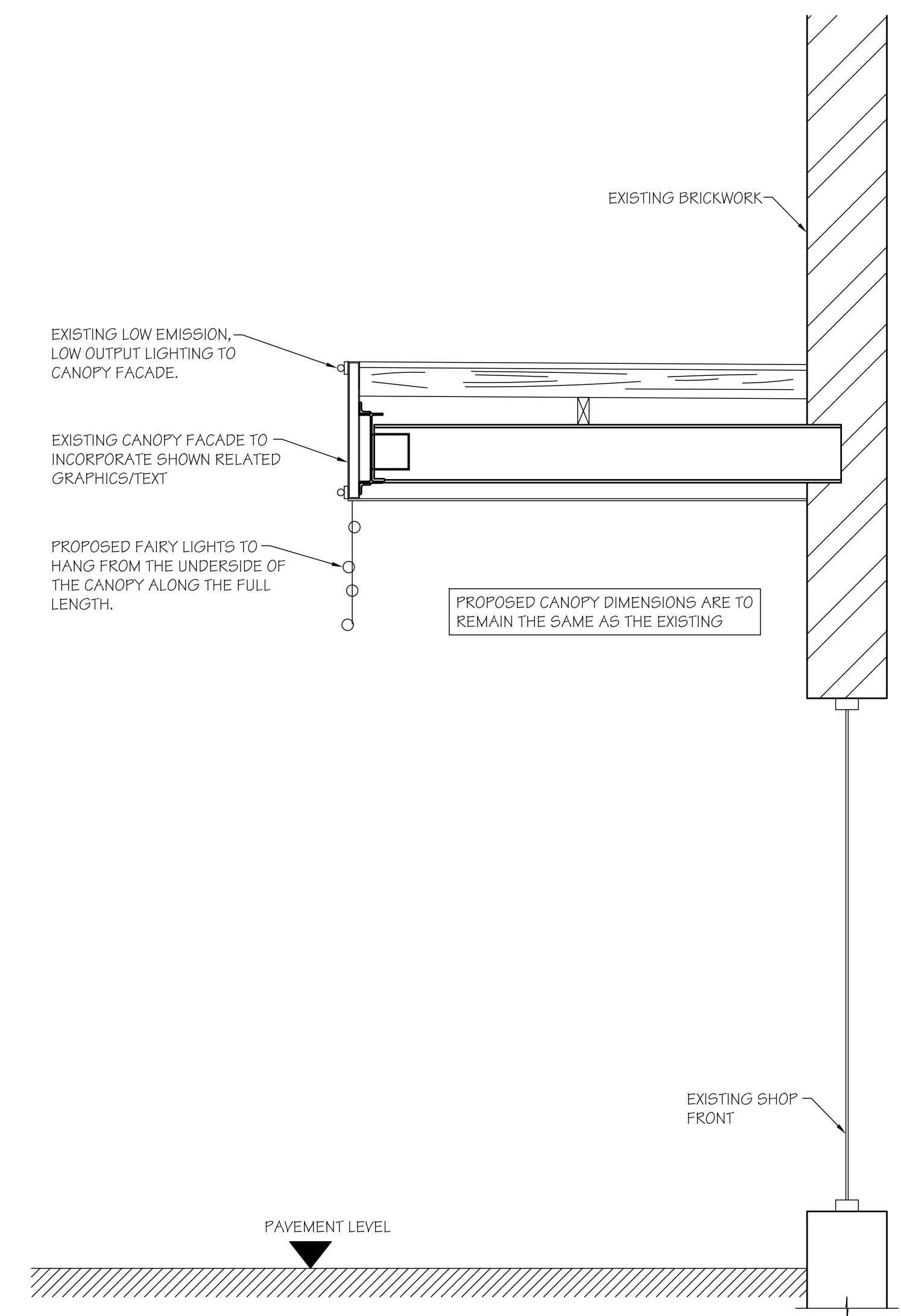
PROPOSED SECTION THROUGH CANOPY (SCALE 1:20 AT A1)
