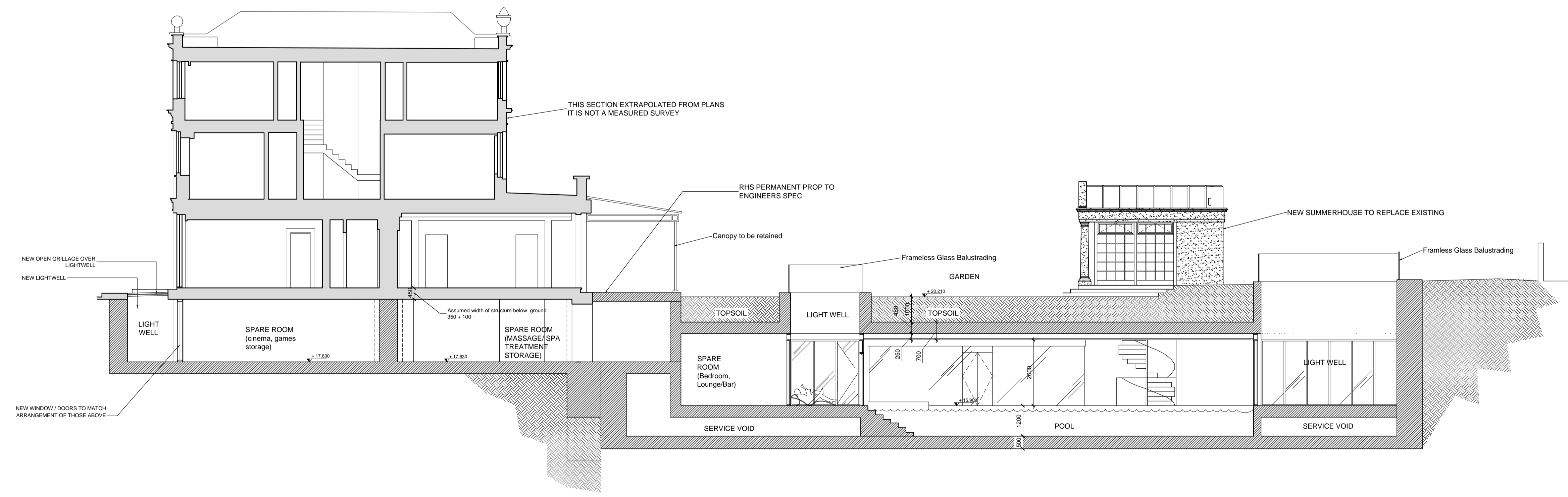
SECTION C-C
