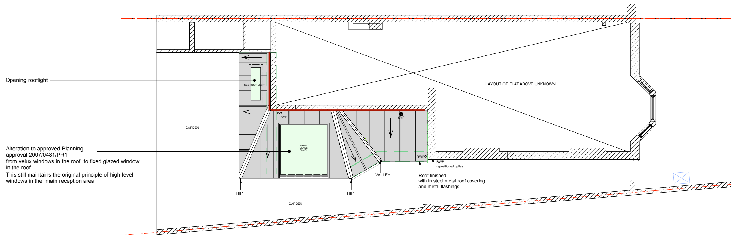
PROPOSED ROOF PLAN
