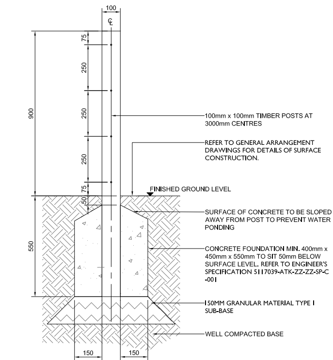
SECTION THROUGH TIMBER POST & WIRE FENCE
