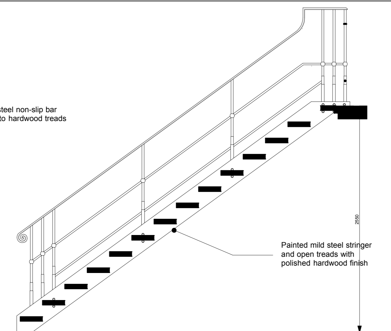
2 Stair Section
