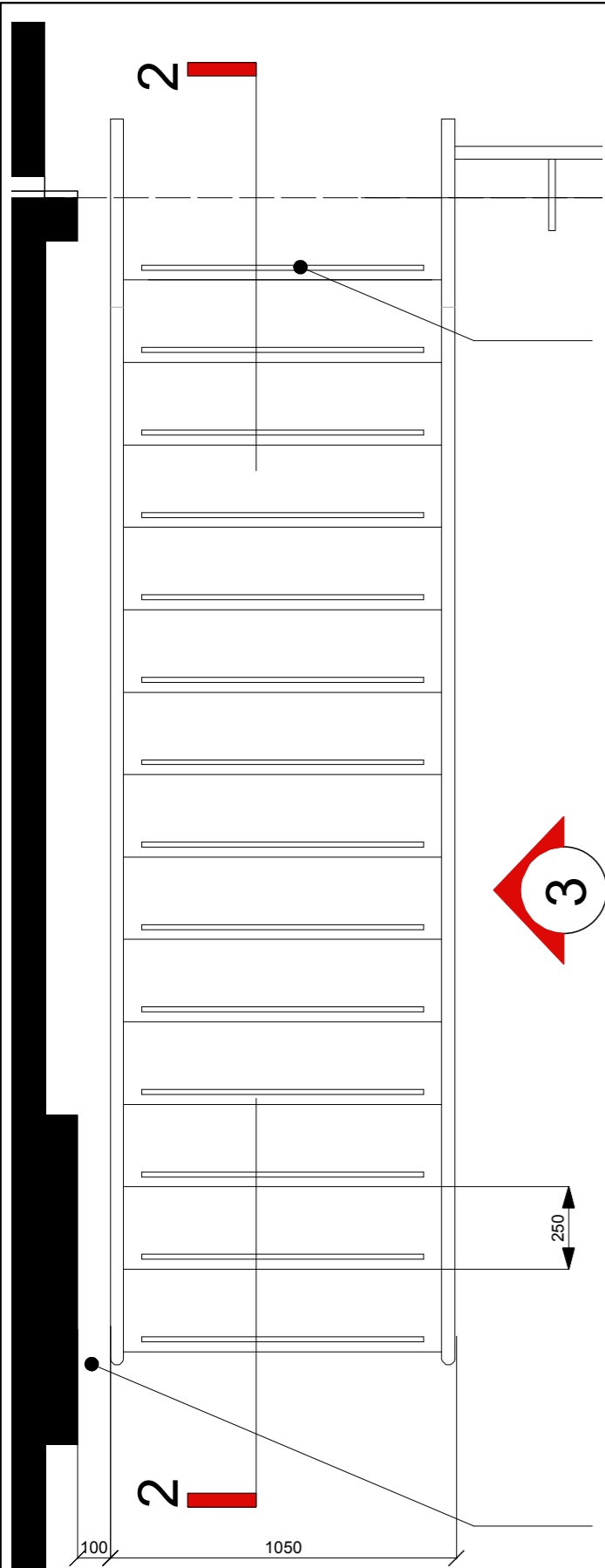
1 Stair Plan
