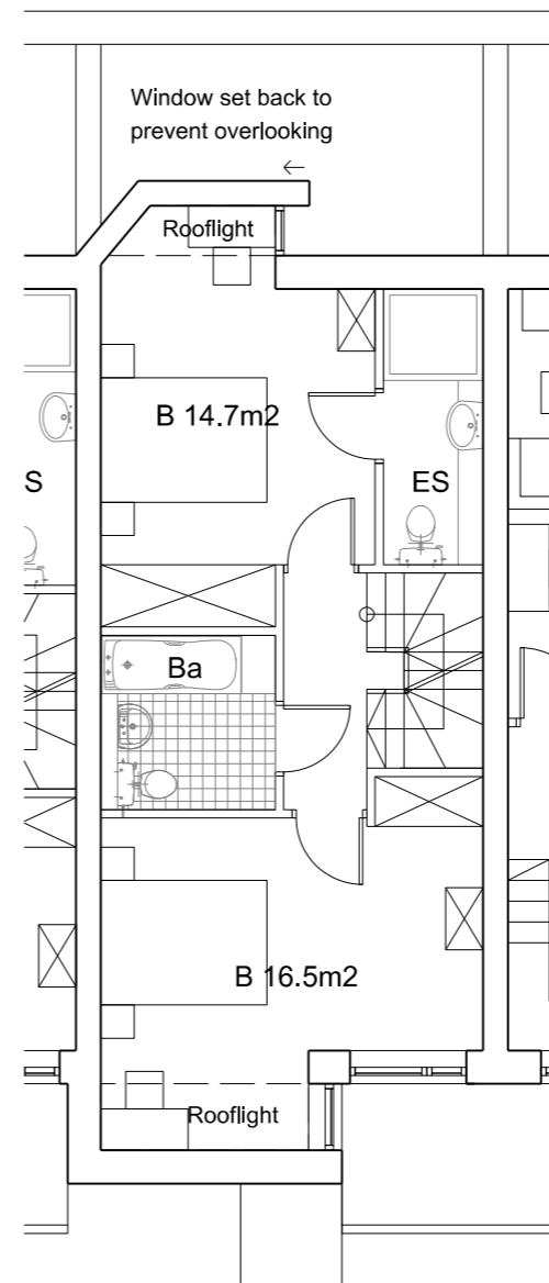
1st FLOOR
