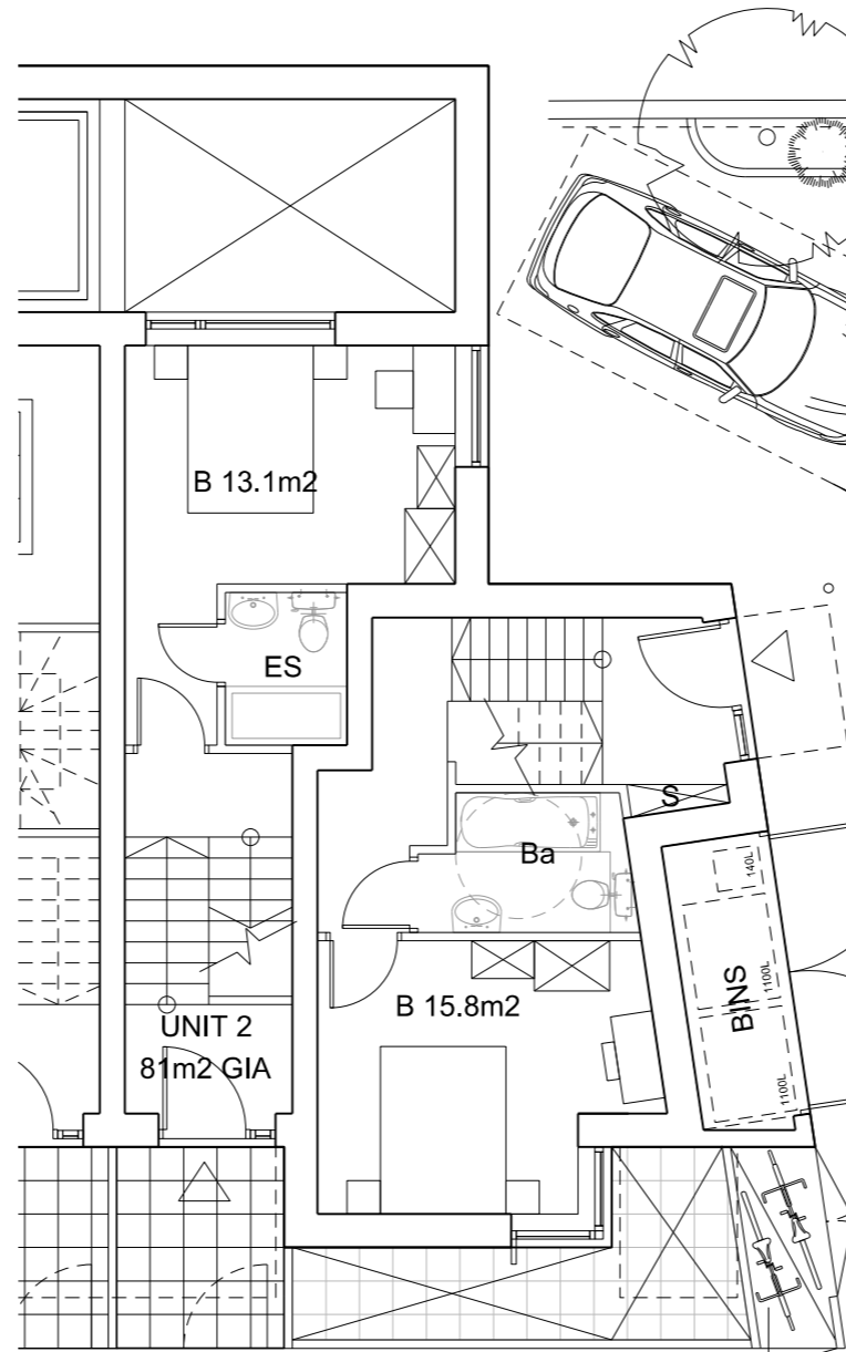
UPPER GROUND FLOOR
