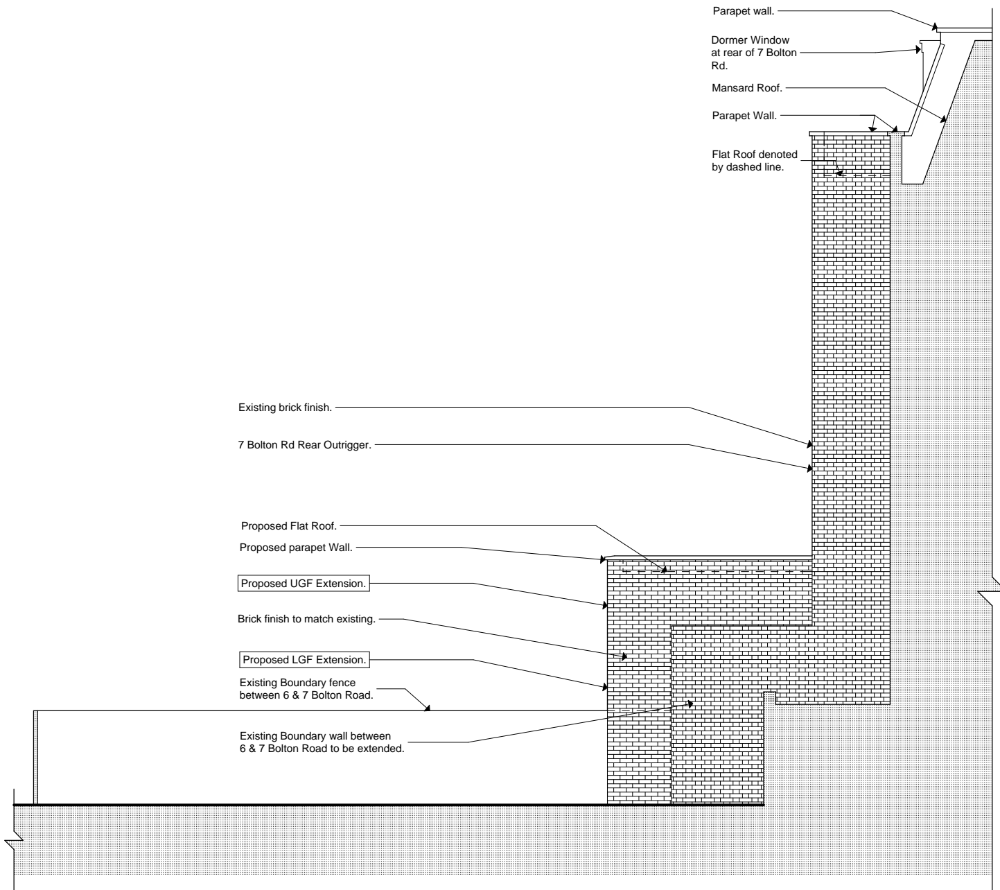
Proposed East Elevation (taken through 6 Bolton Rd)
