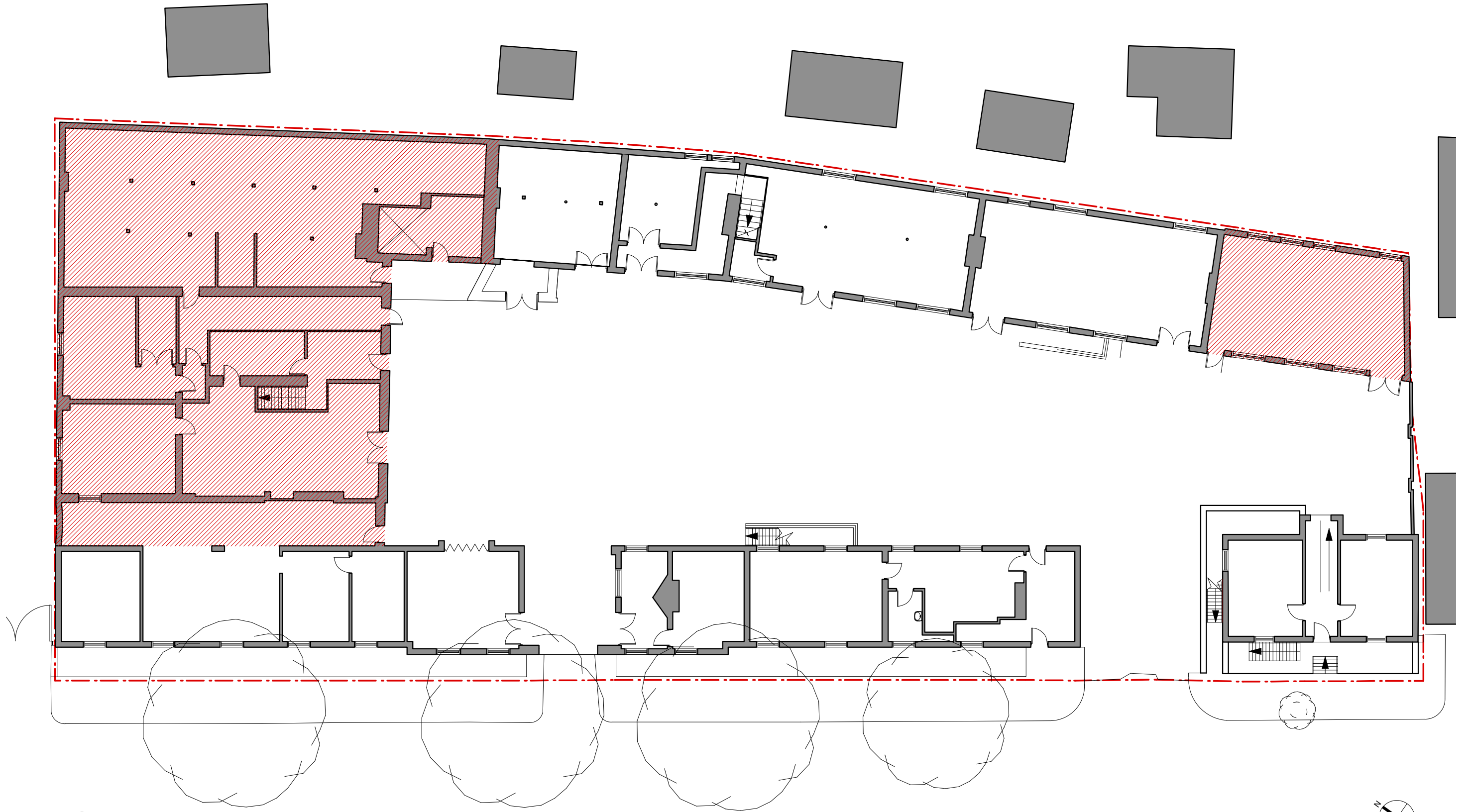
Existing Ground Floor Demolition Drawing DN.00 1:100 @A1 1:200 @A3
