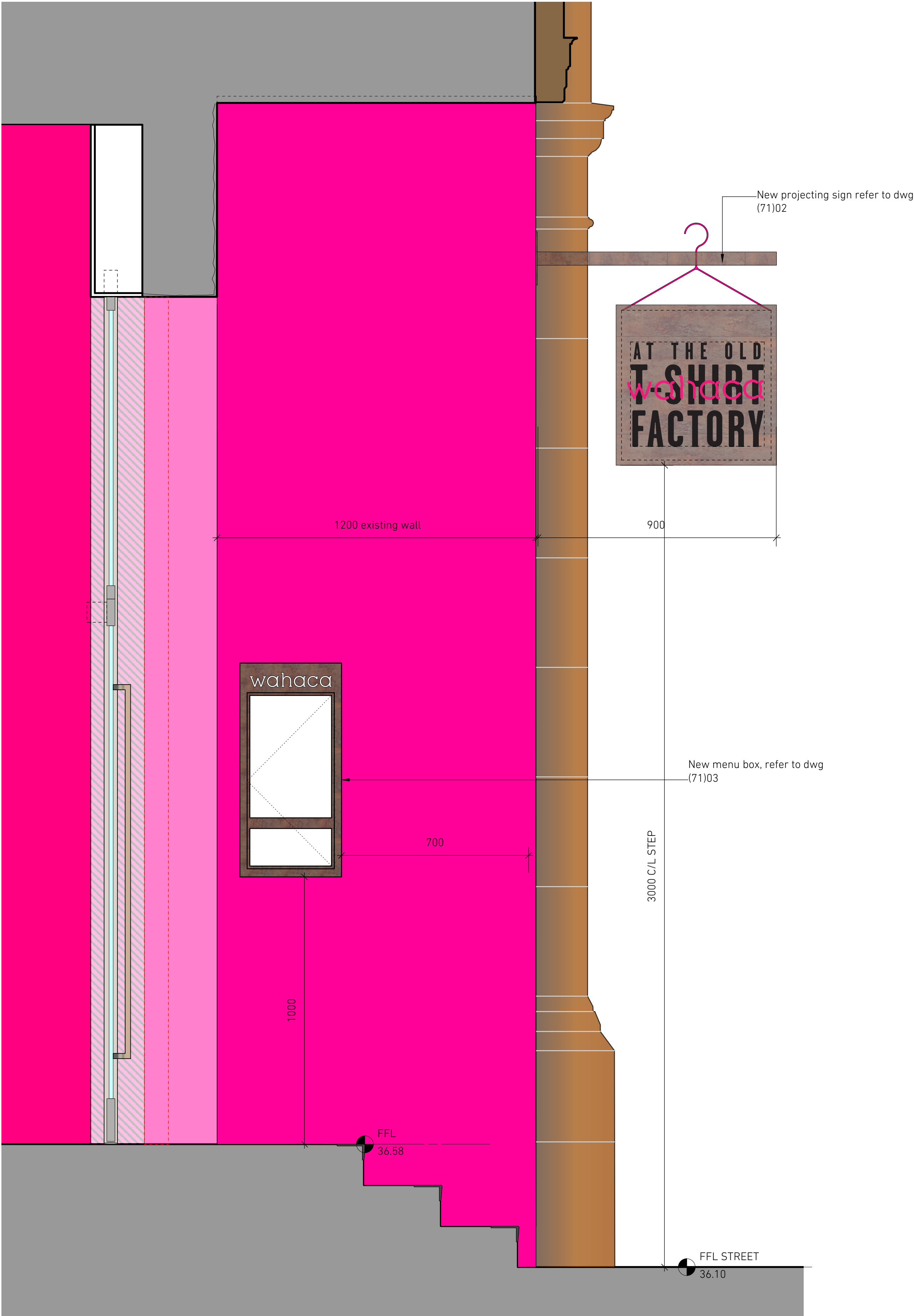
1 PROPOSED ENTRANCE ELEVATION Scale: 1:10
