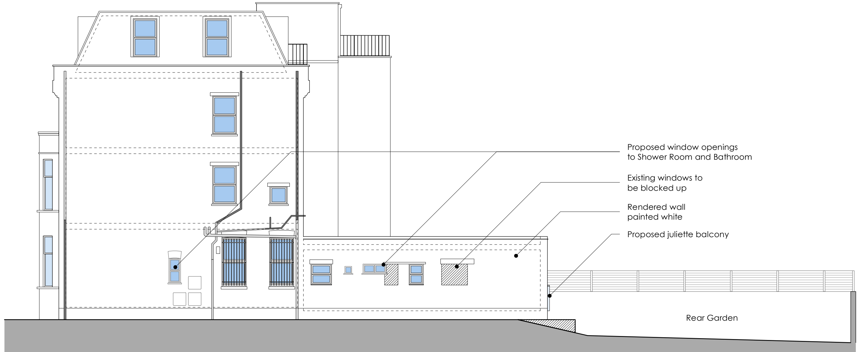
1 P-121 Proposed Side (West) Elevation scale 1:100 @ A3
