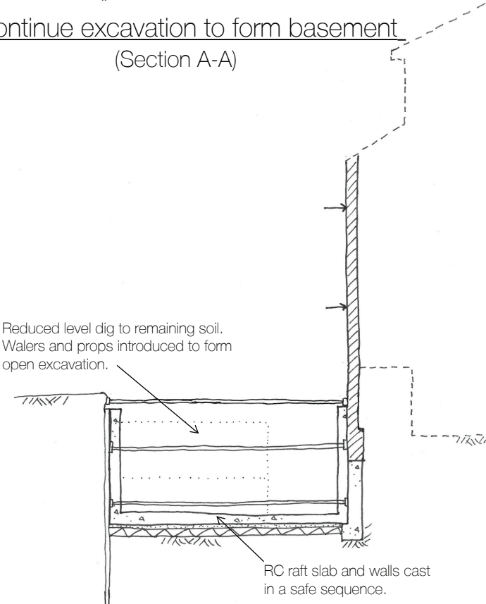
Assumed Sequence of Construction of Basement
