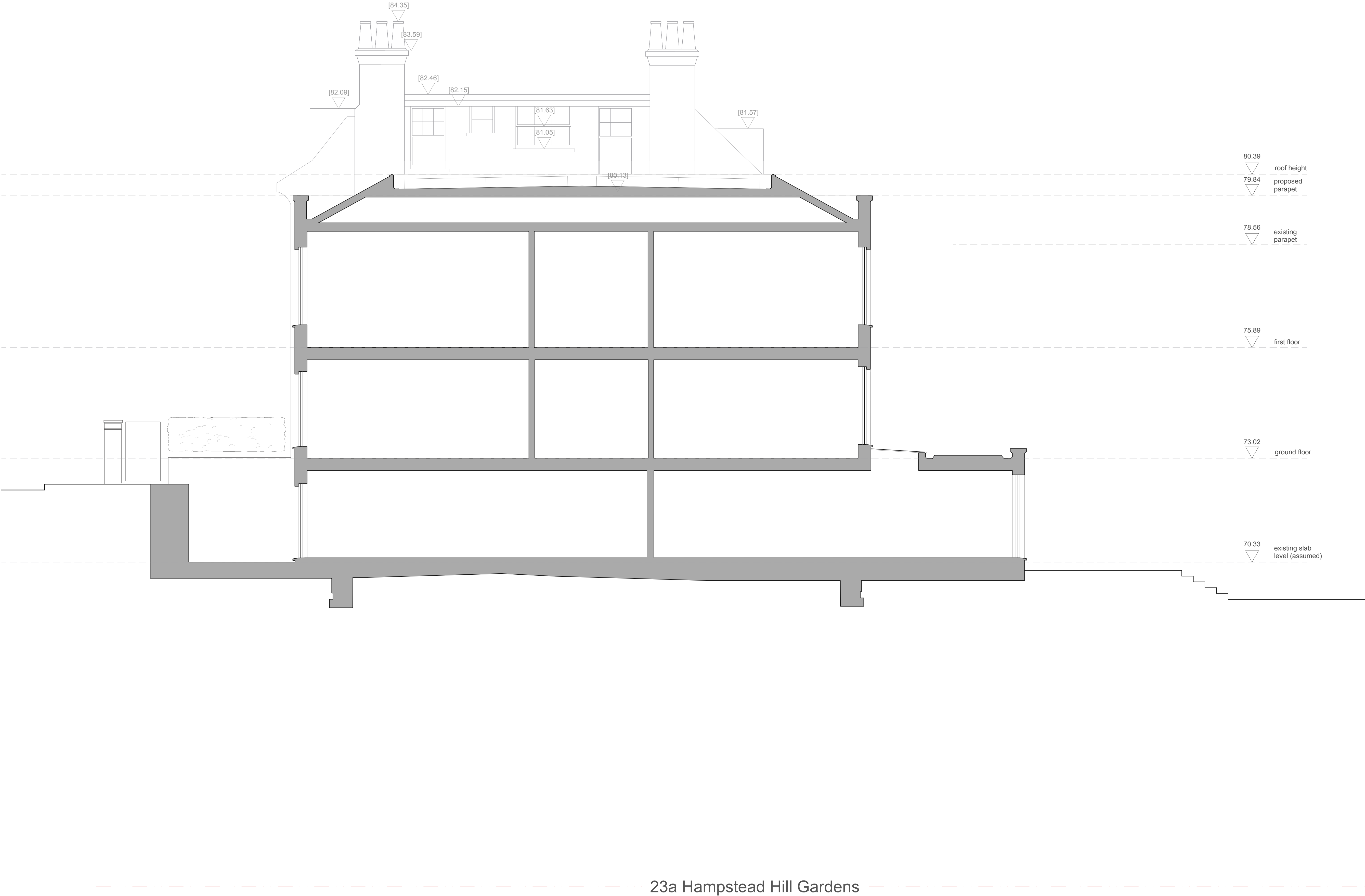
1 Proposed Section AA
