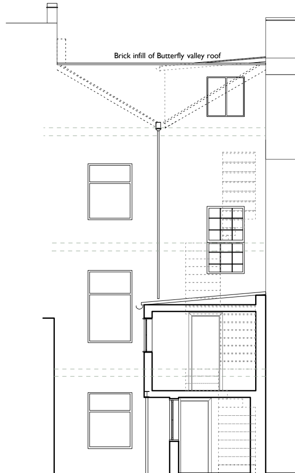
Rear sectionalelevation
