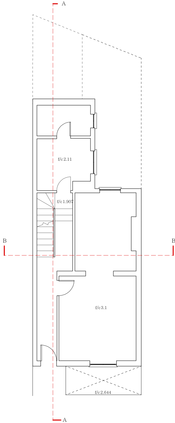
Ground floorPlan
