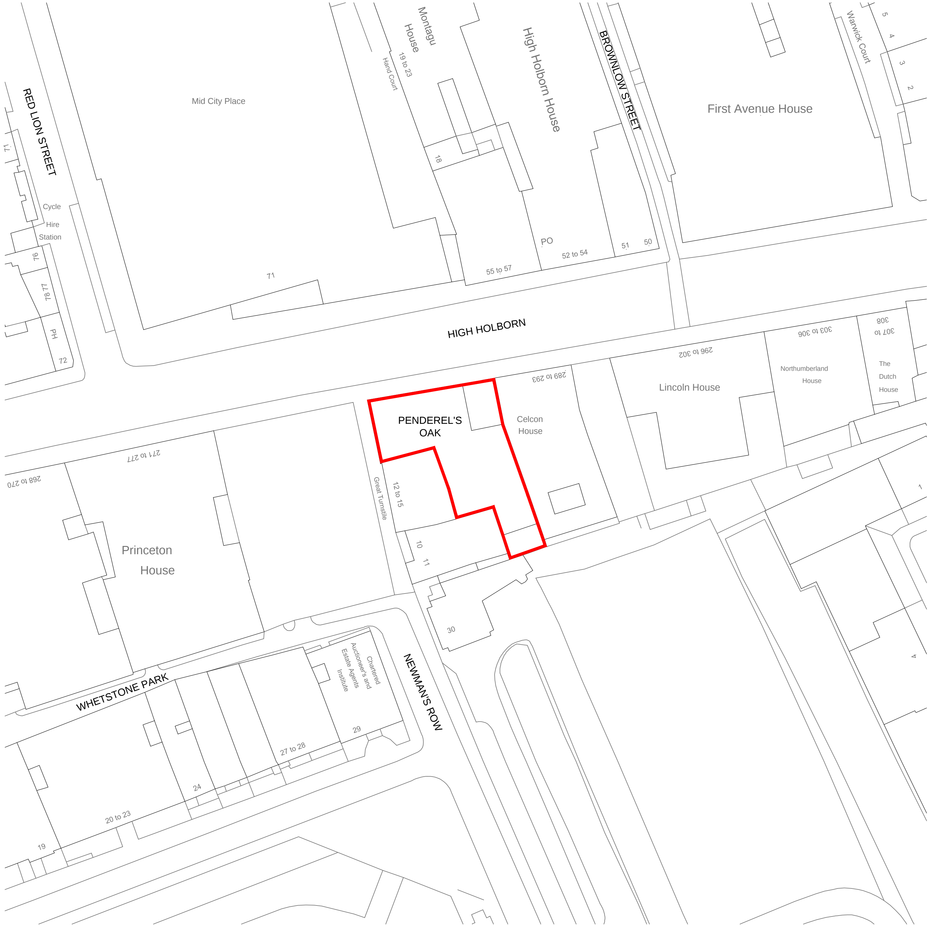
SITE BLOCK PLAN Scale 1:500
