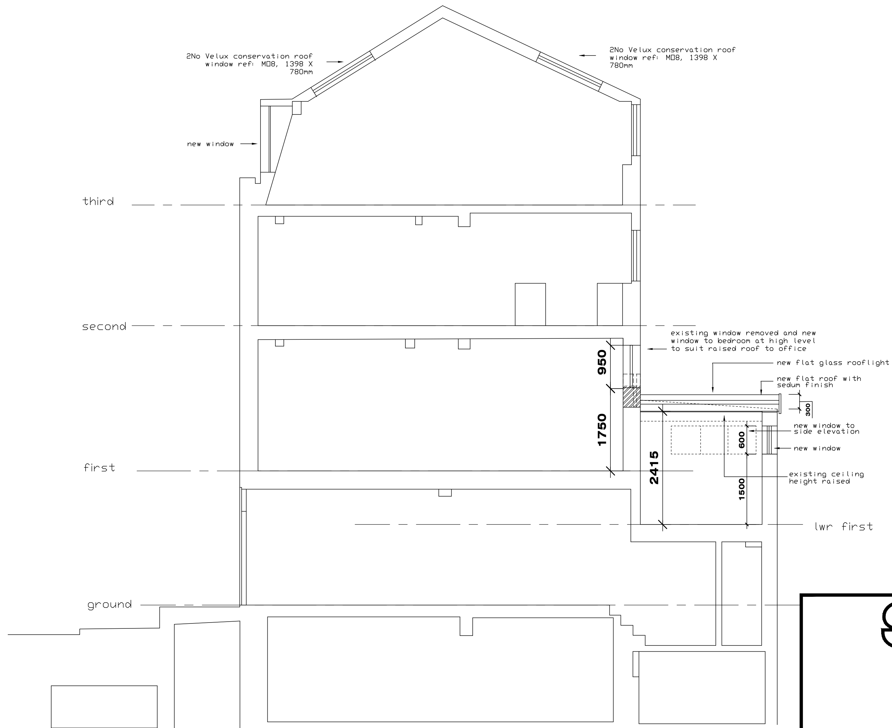
124 PROPOSED SECTION
