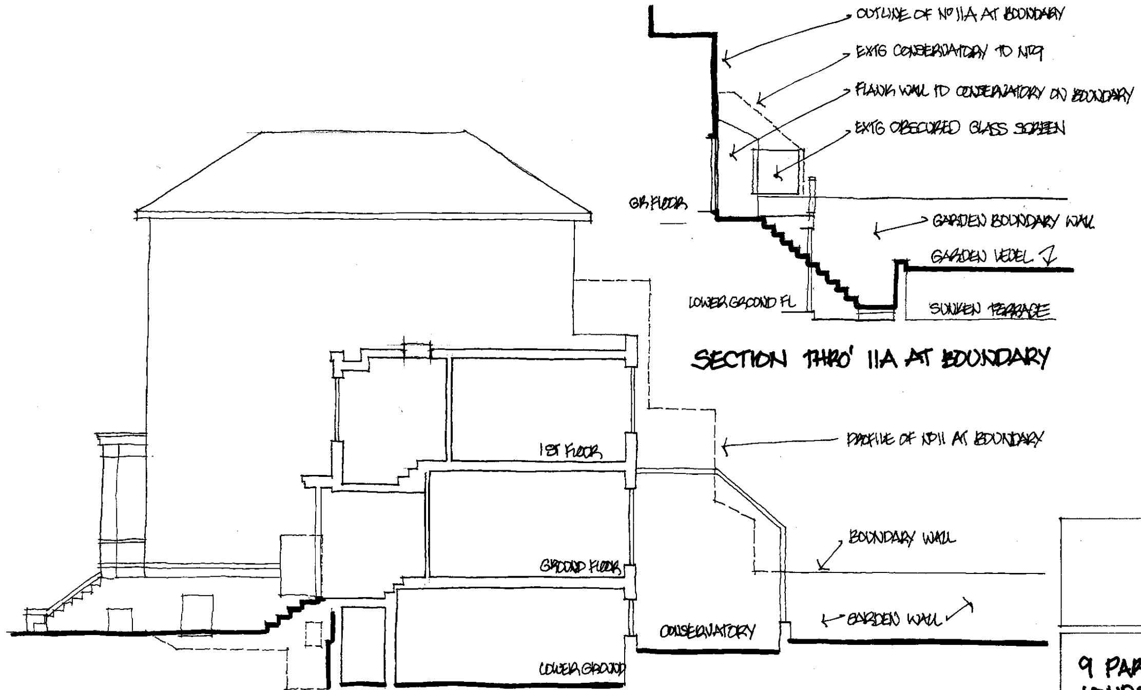
SECTION THRO' COACHHOUSE
