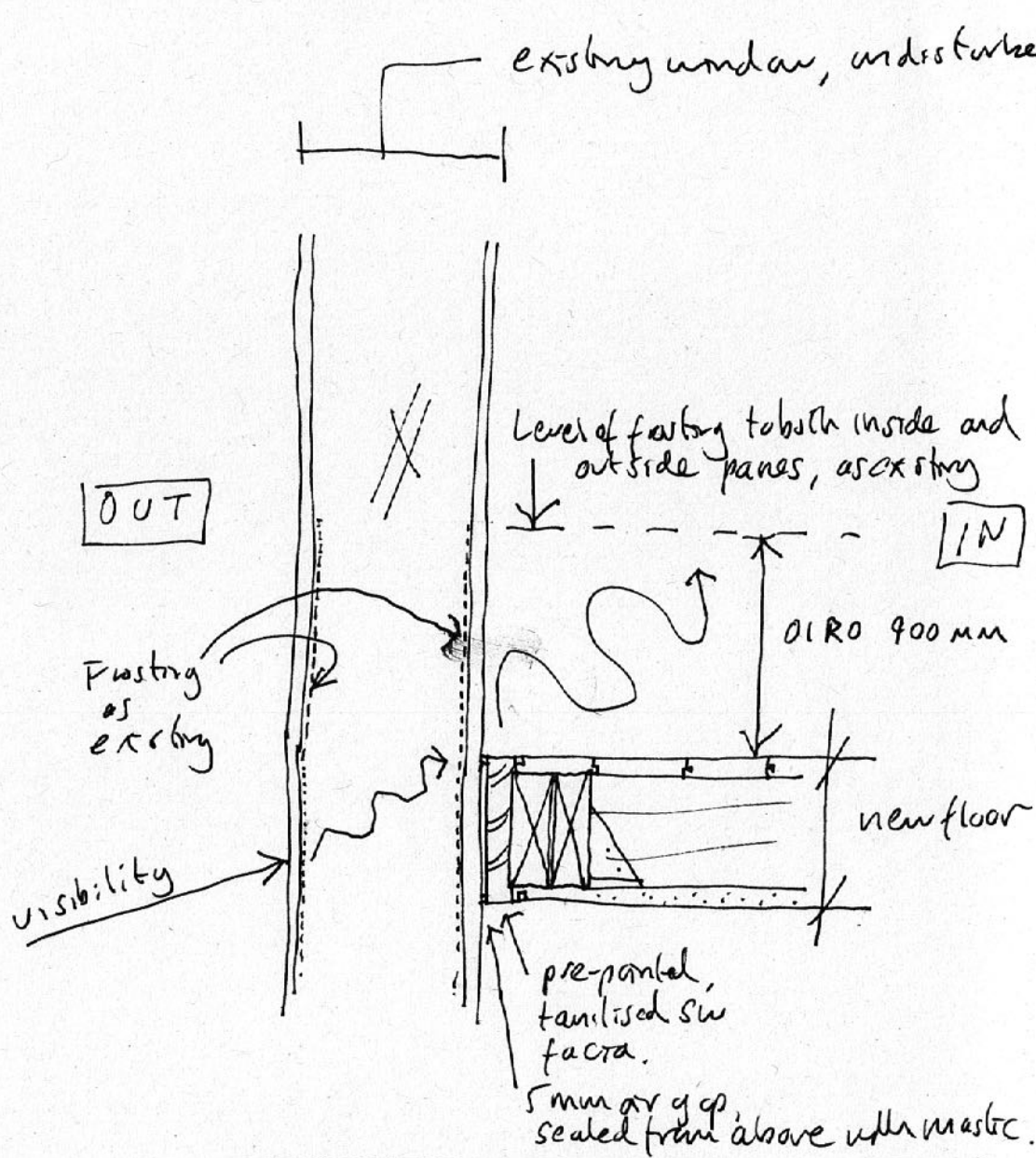
Section N.T.S. through front window + new floor
