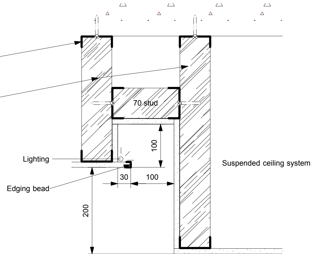
Ceiling Step Lighting Detail
