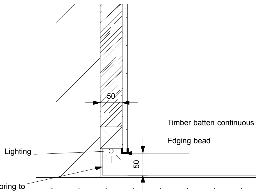
Boundary Skirting Lighting Detail
