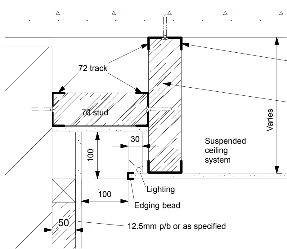
Boundary Lighting Detail
