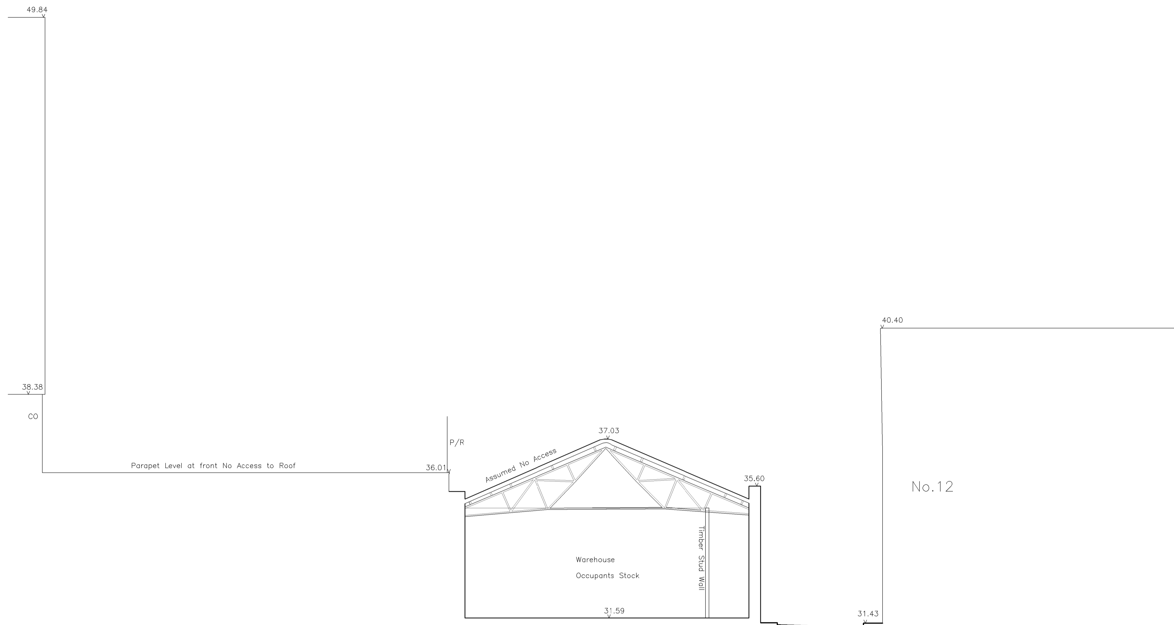
Existing Section A- A 1:100 @ A1
