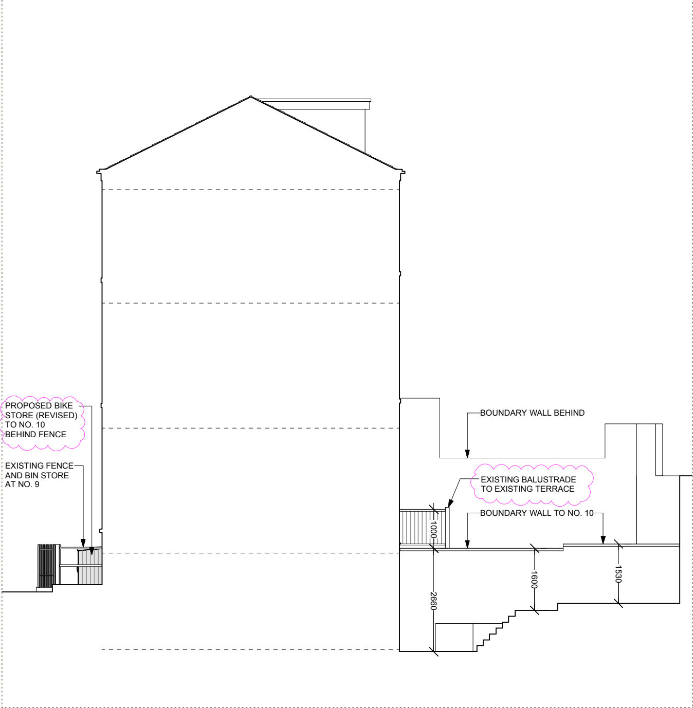
PROPOSED SIDE ELEVATION (VIEWED FROM NO. 9 SHARPLESHALL ST) @ SCALE 1:100
