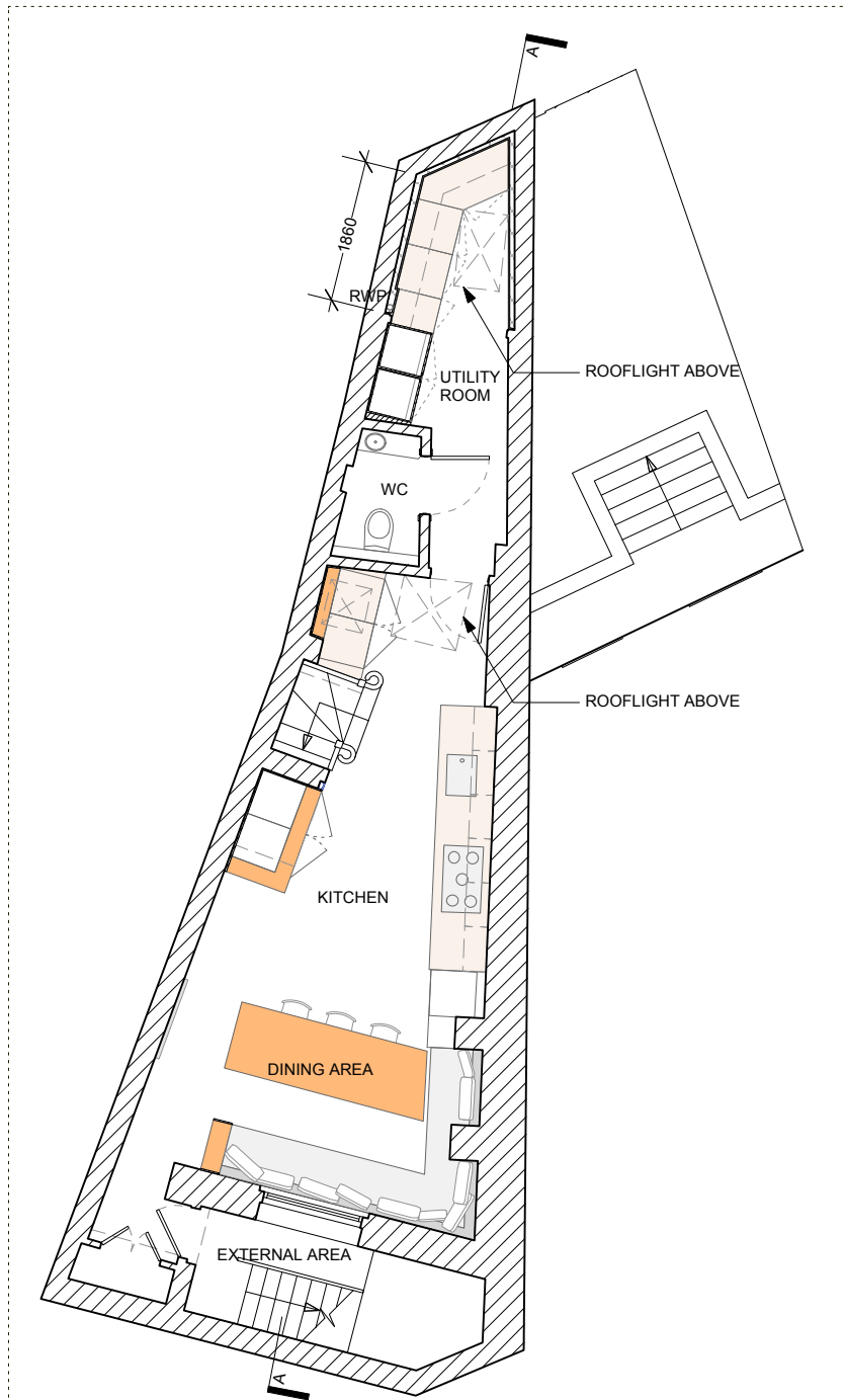
PROPOSED LOWER GROUND FLOOR PLAN
