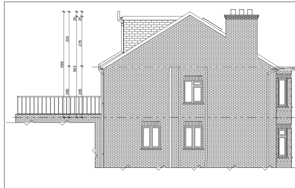
SIDE ELEVATION
