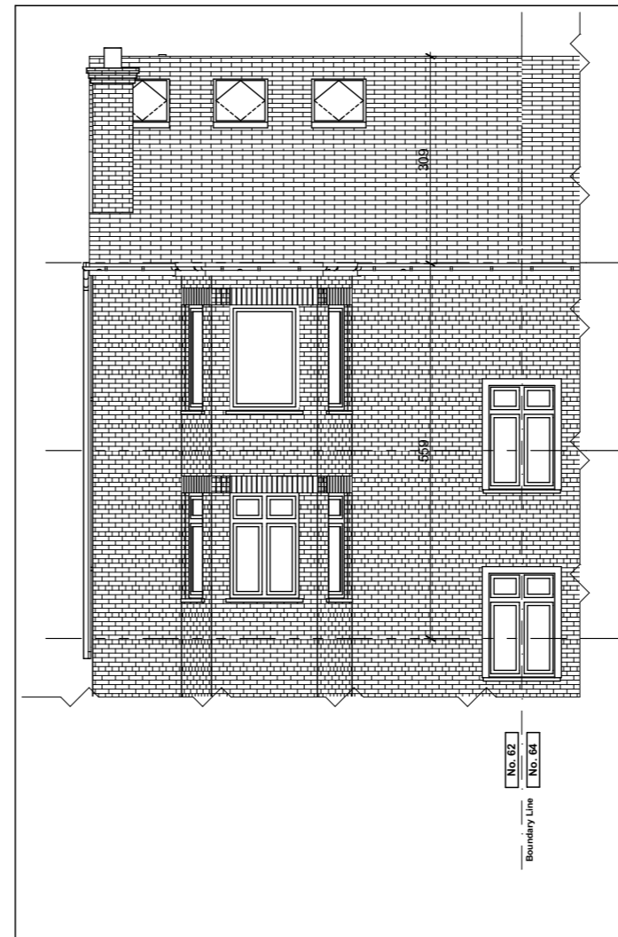
FRONT ELEVATION
