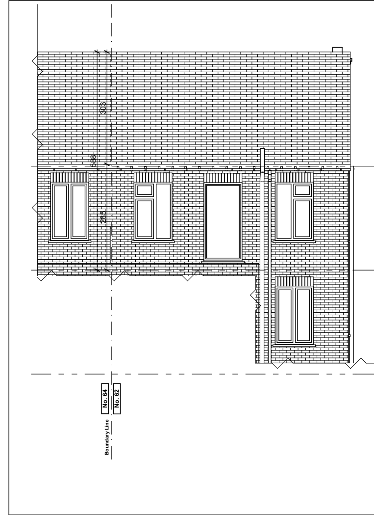
REAR ELEVATION
