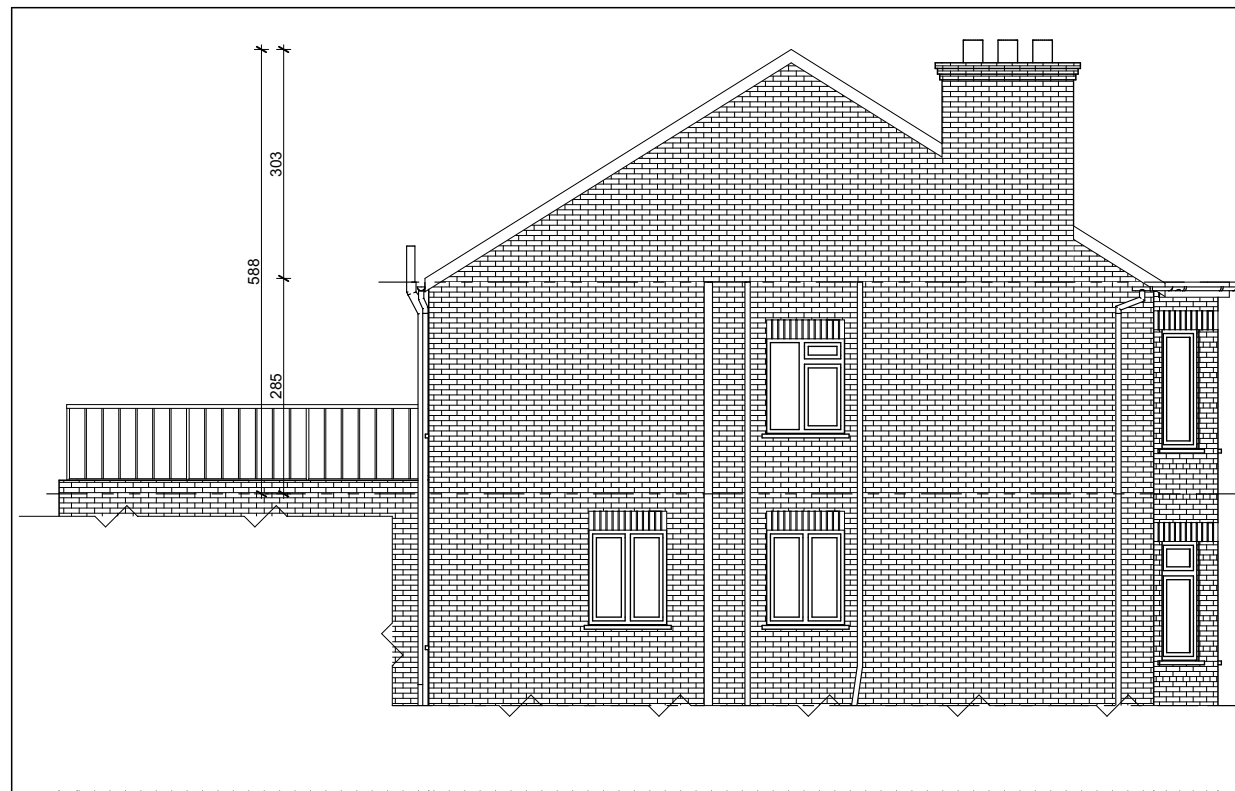
SIDE ELEVATION
