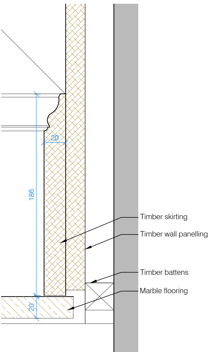
04 - PROPOSED SKIRTING DETAIL
