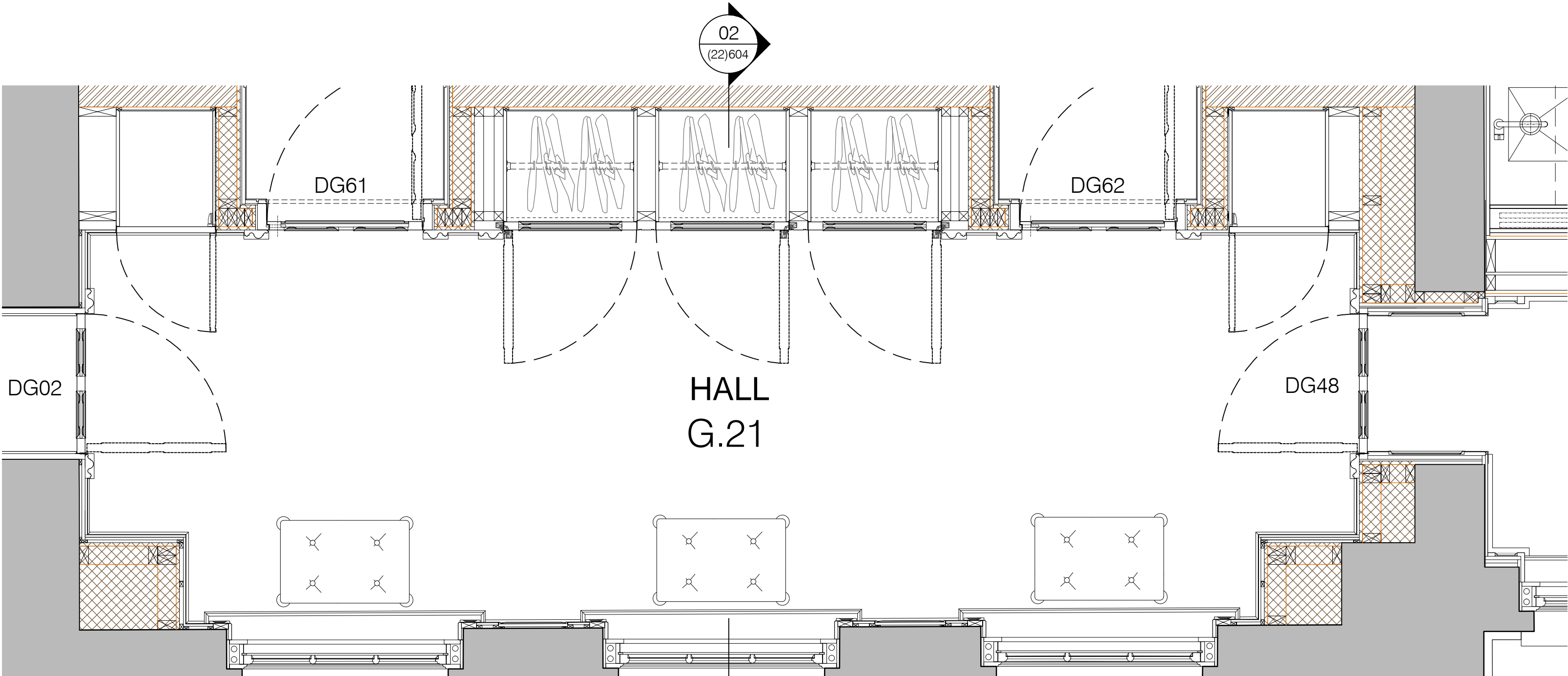
03 - PLAN OF G.21
