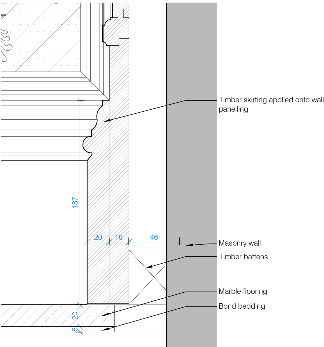
04 - PROPOSED SKIRTING DETAIL
