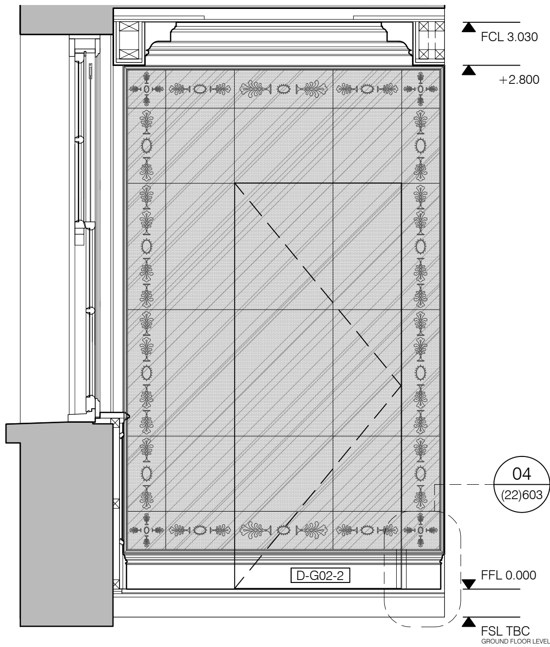
03 - SECTION THROUGH G.02
