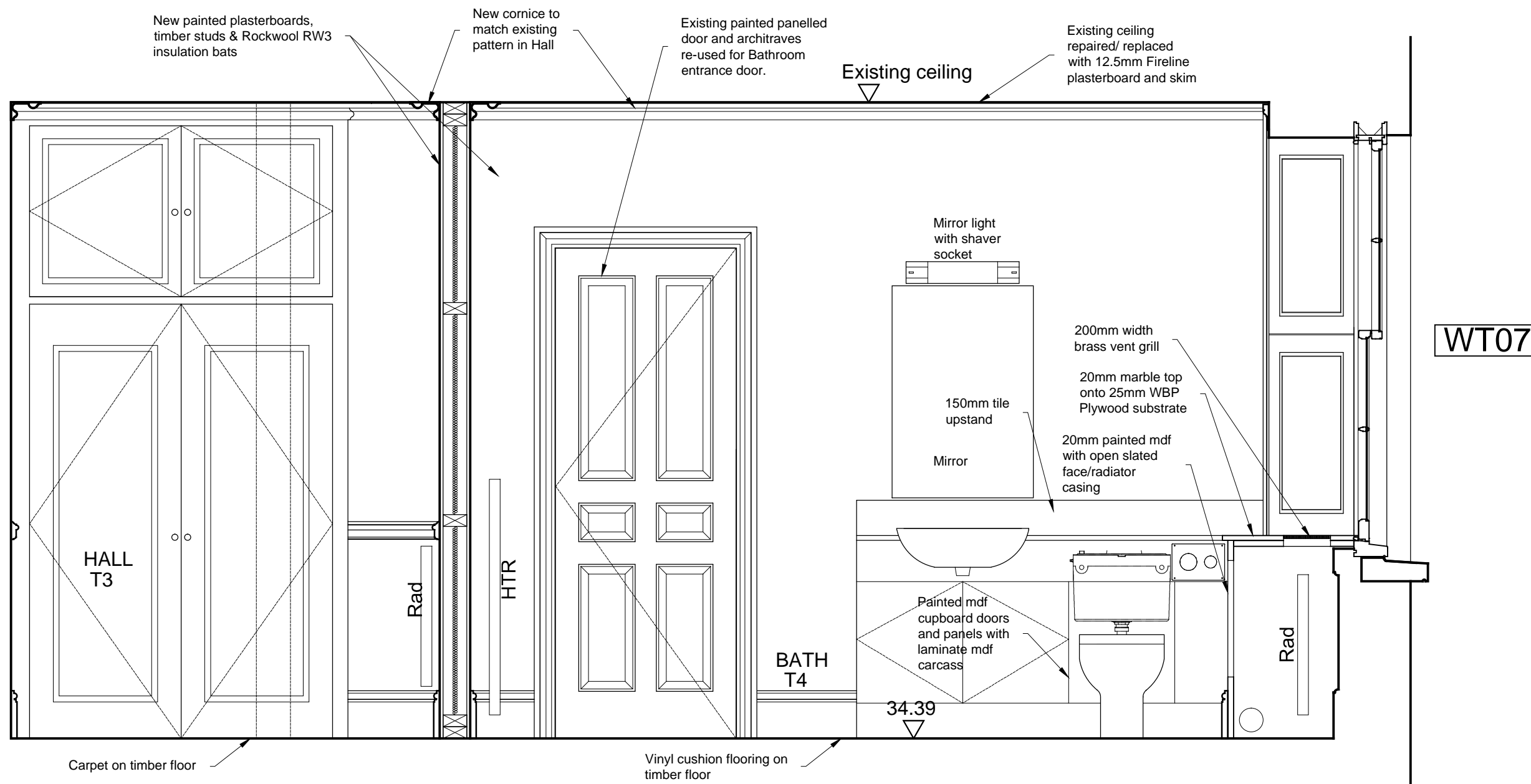
PROPOSED BATHROOM SOUTH ELEVATION
