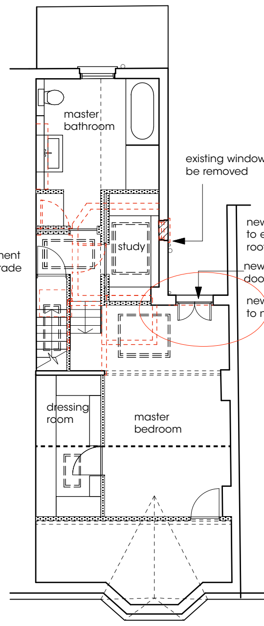
Second Floor
