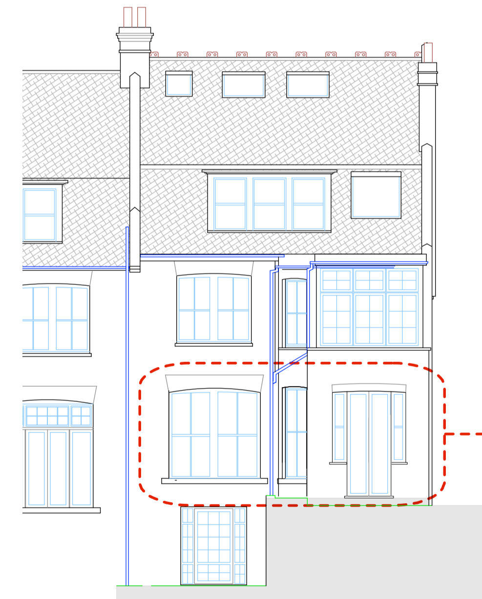
REAR(SOUTH WEST)
