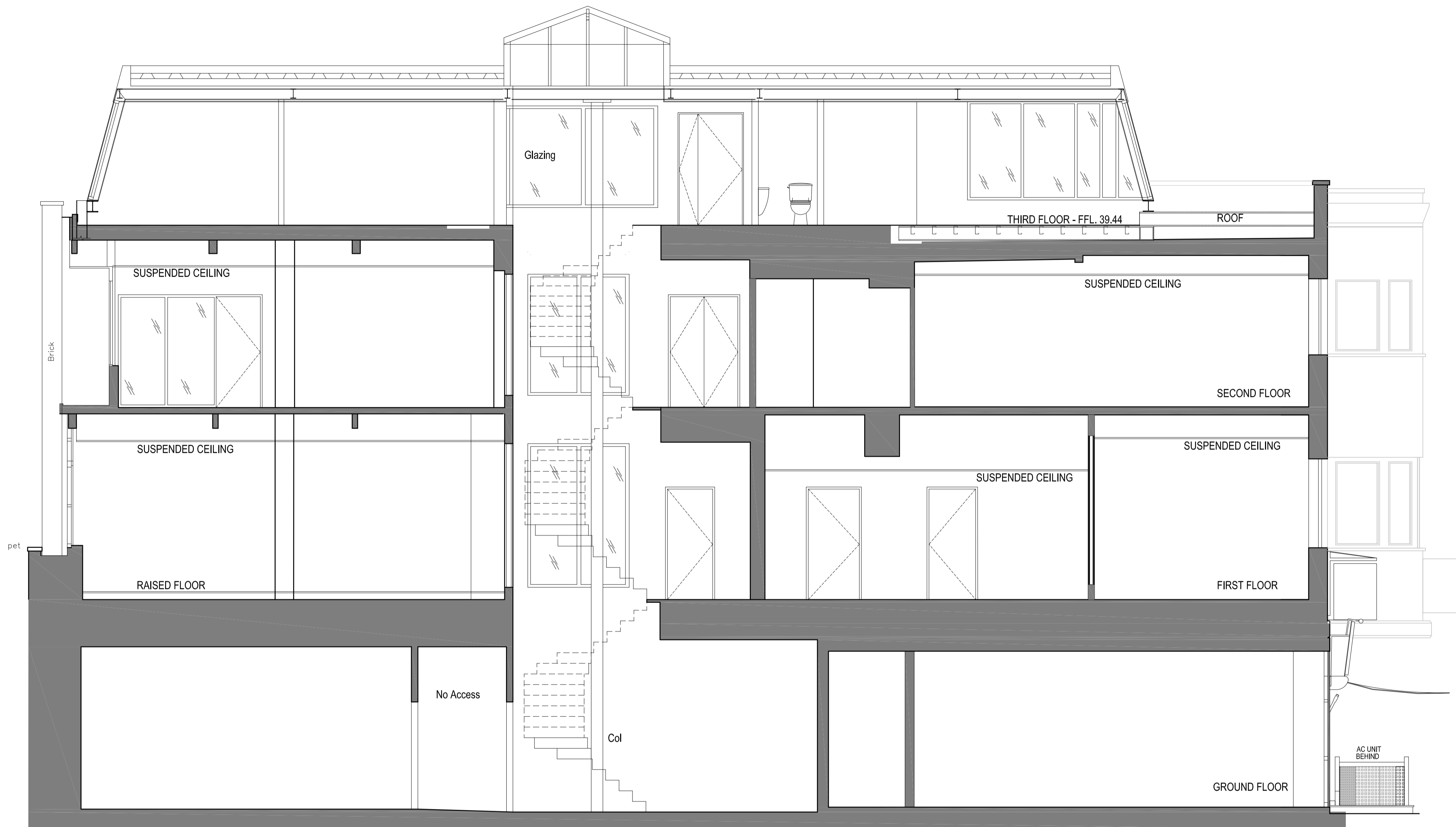
1 EXISTING SECTION AA
