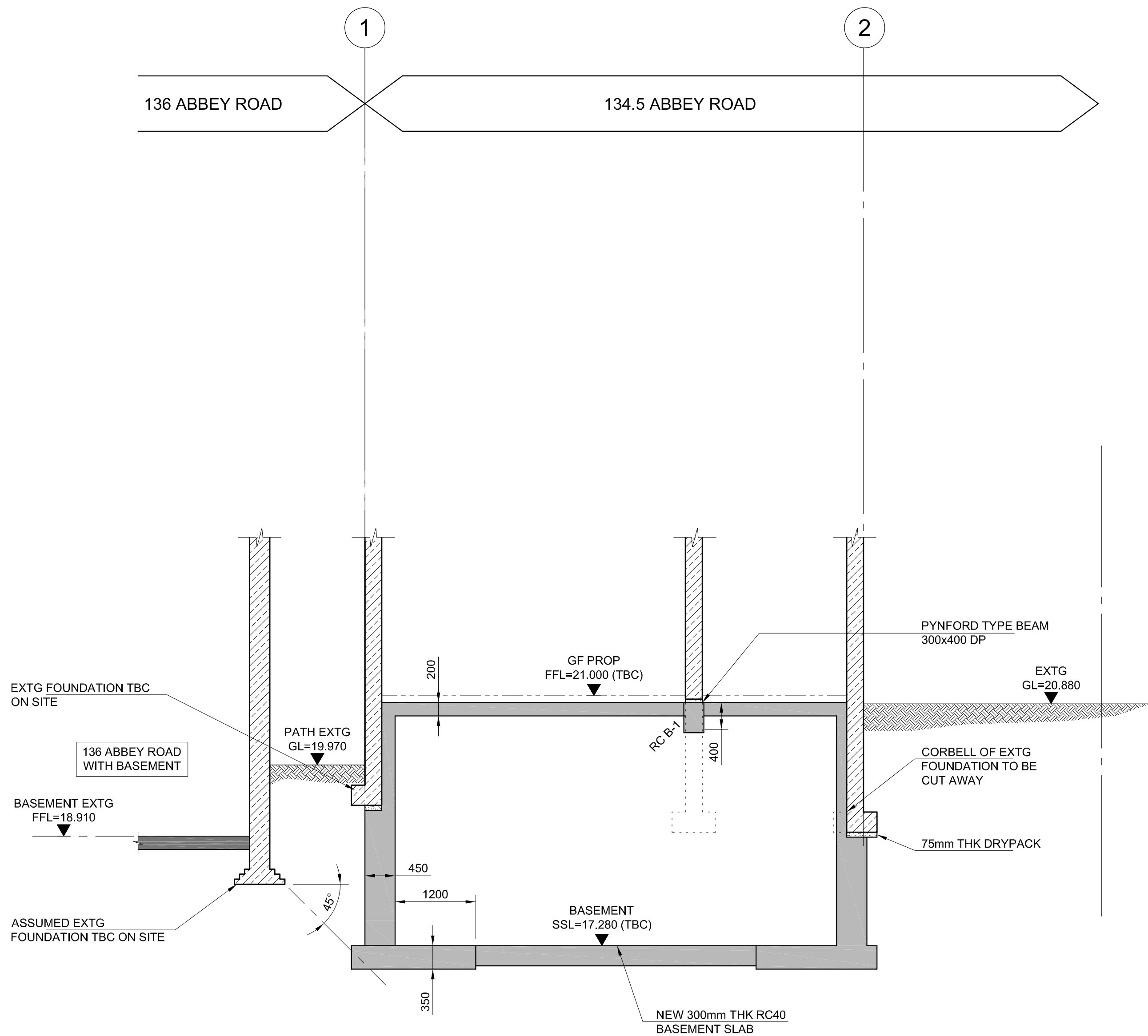
PROPOSED SECTION B 1:50 @ A1
