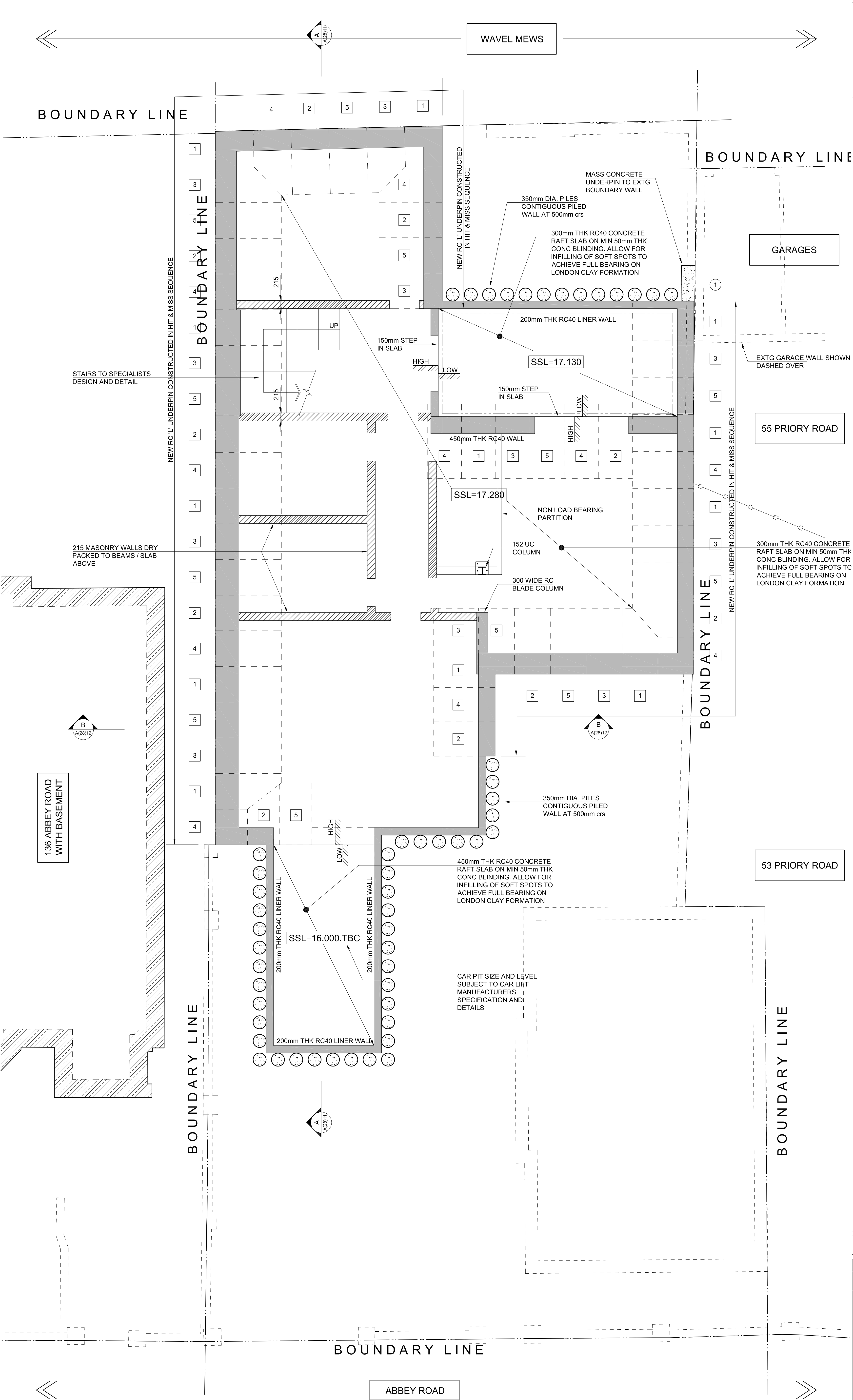
PROPOSED BASEMENT PLAN
