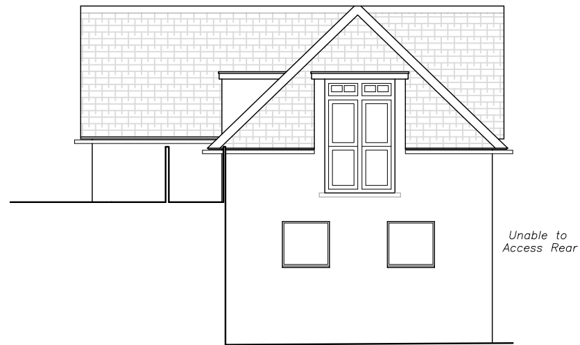
NORTH EAST ELEVATION 1 1:100 @ A3 MVL-X2-300
