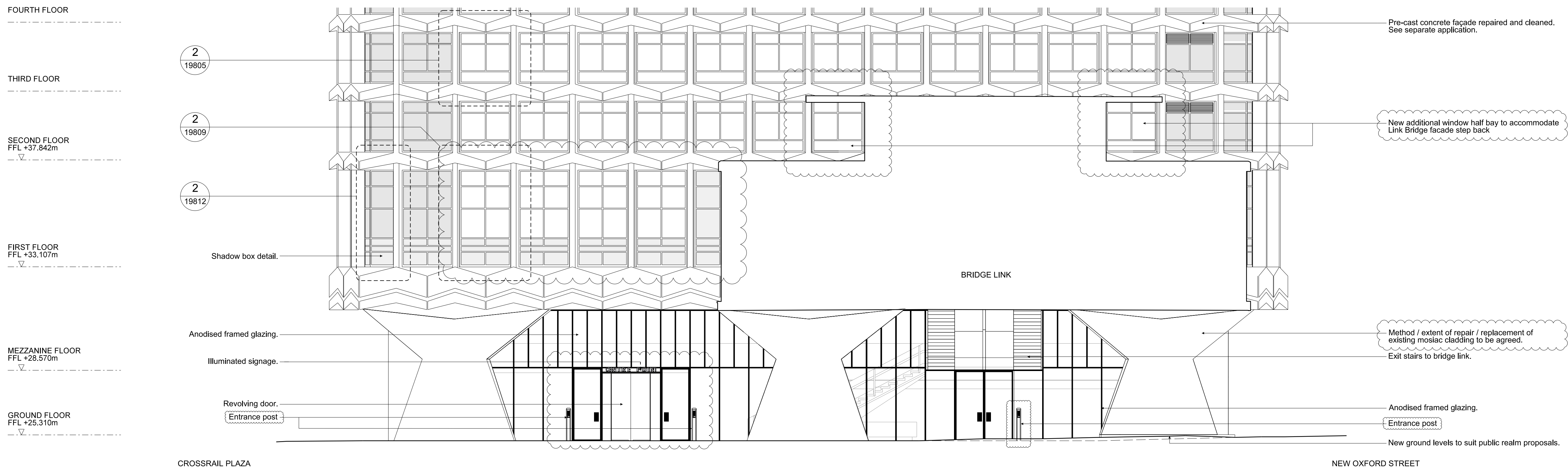
2 ELEVATION EAST PROPOSED 1:100 LOWER LEVELS
