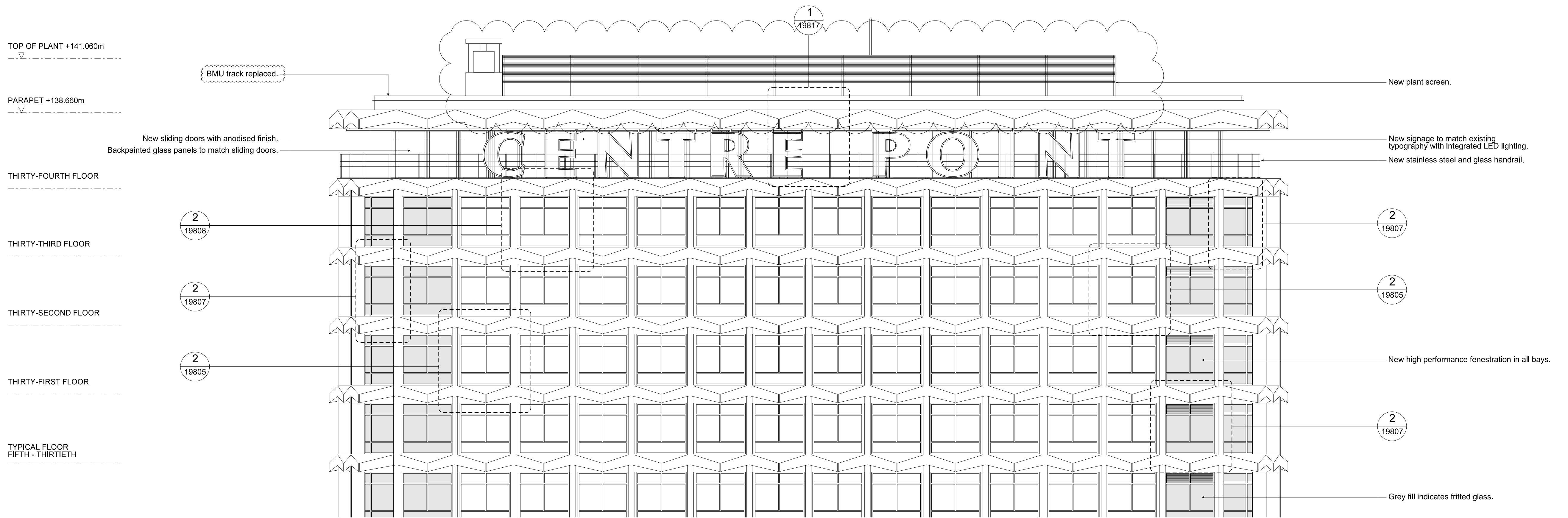
1 ELEVATION EAST PROPOSED 1:100 UPPER LEVELS
