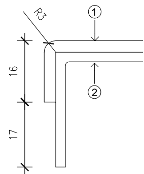
Plan Detail SCALE 1:1
